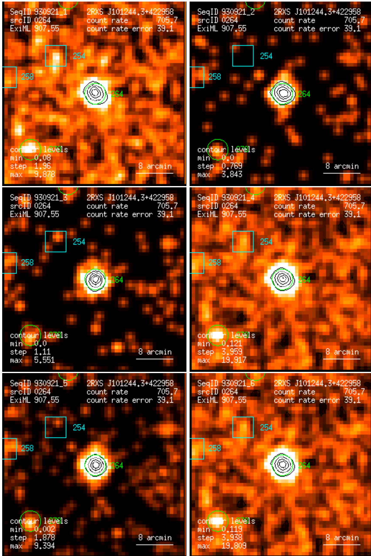
Figure 264: RASS 930921: detection 0264: band rate images, Gaussian filter: (1) PSPC channels 11 – 41, (2) 52 – 90, (3) 91 – 201, (4) 11 – 235, (5) 52 – 201, (6) 11 – 201. Broad band rates in counts/ks. Band rate contour levels in counts/ks/arcmin 2 .
