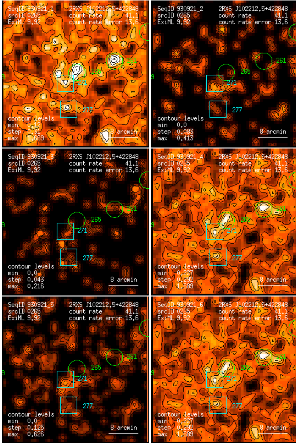
Figure 265: RASS 930921: detection 0265: band rate images, Gaussian filter: (1) PSPC channels 11 – 41, (2) 52 – 90, (3) 91 – 201, (4) 11 – 235, (5) 52 – 201, (6) 11 – 201. Broad band rates in counts/ks. Band rate contour levels in counts/ks/arcmin 2 .
