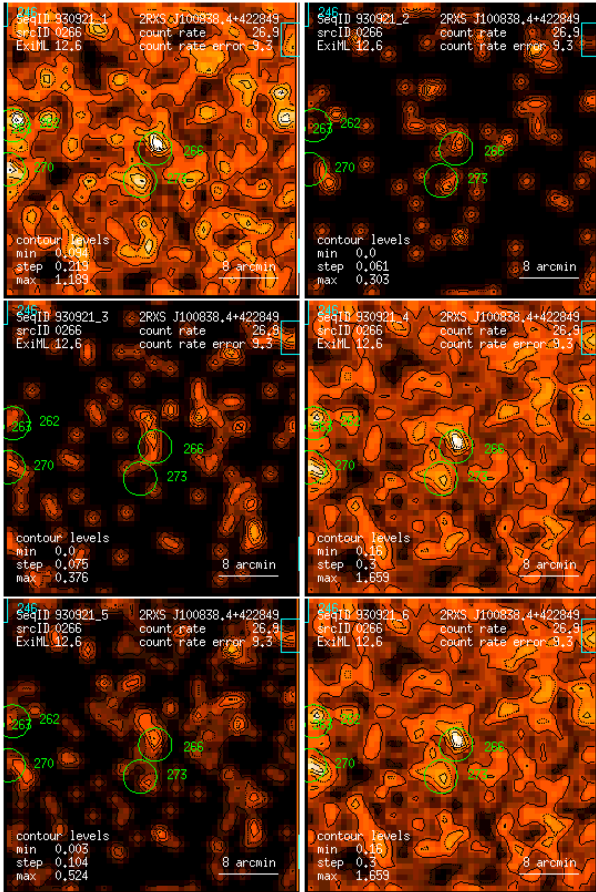
Figure 266: RASS 930921: detection 0266: band rate images, Gaussian filter: (1) PSPC channels 11 – 41, (2) 52 – 90, (3) 91 – 201, (4) 11 – 235, (5) 52 – 201, (6) 11 – 201. Broad band rates in counts/ks. Band rate contour levels in counts/ks/arcmin 2 .
