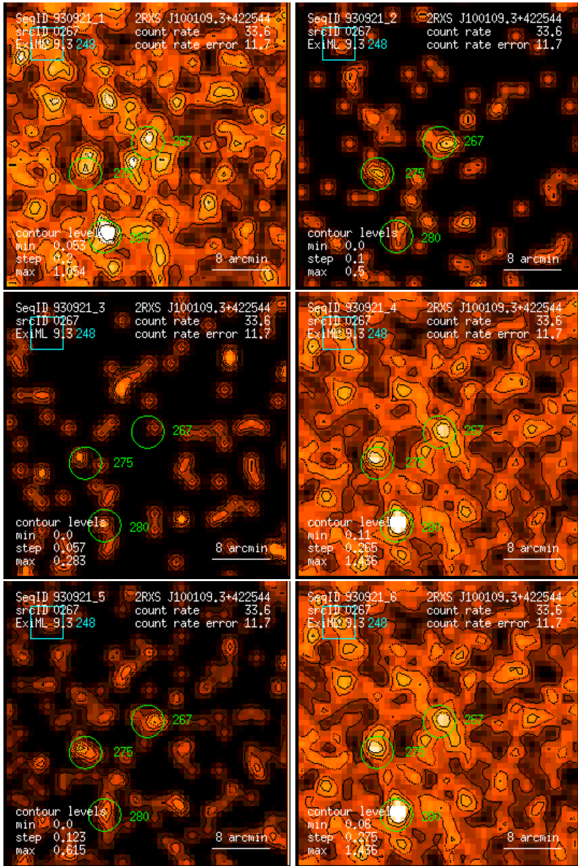
Figure 267: RASS 930921: detection 0267: band rate images, Gaussian filter: (1) PSPC channels 11 – 41, (2) 52 – 90, (3) 91 – 201, (4) 11 – 235, (5) 52 – 201, (6) 11 – 201. Broad band rates in counts/ks. Band rate contour levels in counts/ks/arcmin 2 .
