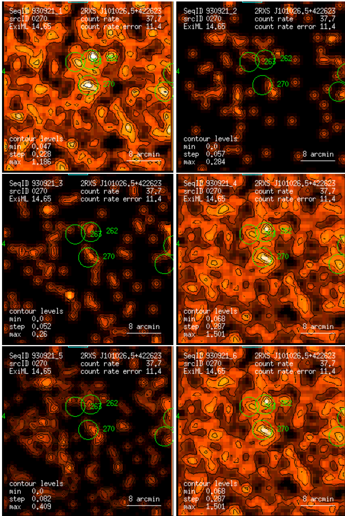
Figure 270: RASS 930921: detection 0270: band rate images, Gaussian filter: (1) PSPC channels 11 – 41, (2) 52 – 90, (3) 91 – 201, (4) 11 – 235, (5) 52 – 201, (6) 11 – 201. Broad band rates in counts/ks. Band rate contour levels in counts/ks/arcmin 2 .
