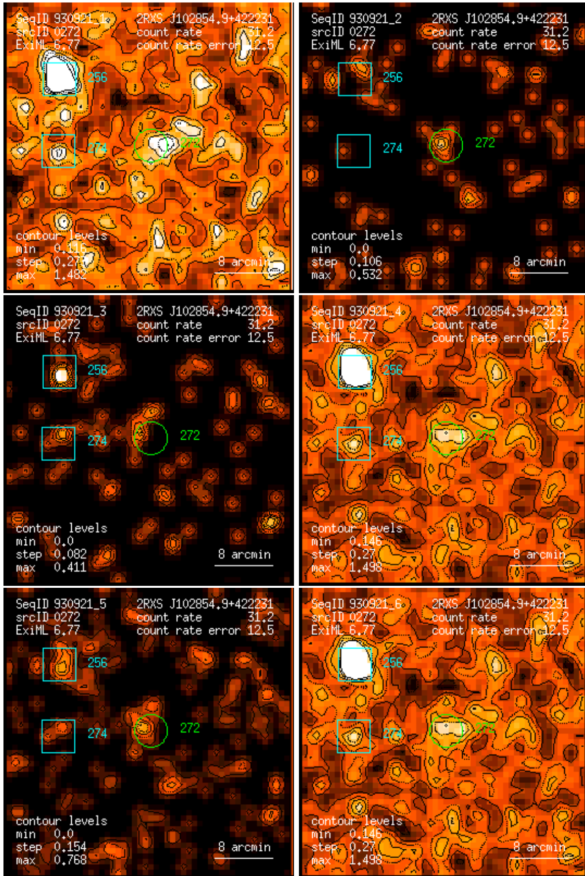
Figure 272: RASS 930921: detection 0272: band rate images, Gaussian filter: (1) PSPC channels 11 – 41, (2) 52 – 90, (3) 91 – 201, (4) 11 – 235, (5) 52 – 201, (6) 11 – 201. Broad band rates in counts/ks. Band rate contour levels in counts/ks/arcmin 2 .
