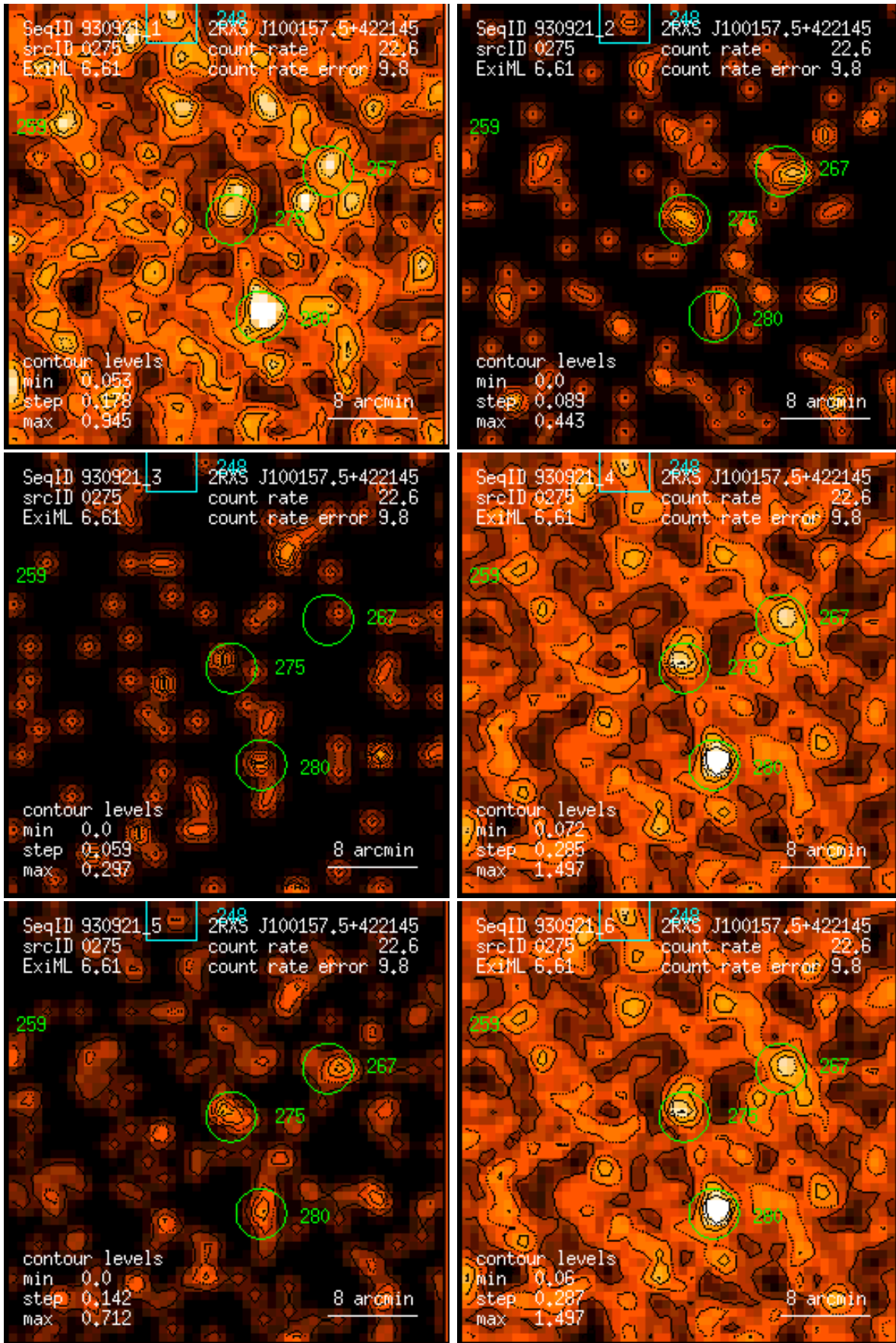
Figure 275: RASS 930921: detection 0275: band rate images, Gaussian filter: (1) PSPC channels 11 – 41, (2) 52 – 90, (3) 91 – 201, (4) 11 – 235, (5) 52 – 201, (6) 11 – 201. Broad band rates in counts/ks. Band rate contour levels in counts/ks/arcmin 2 .
