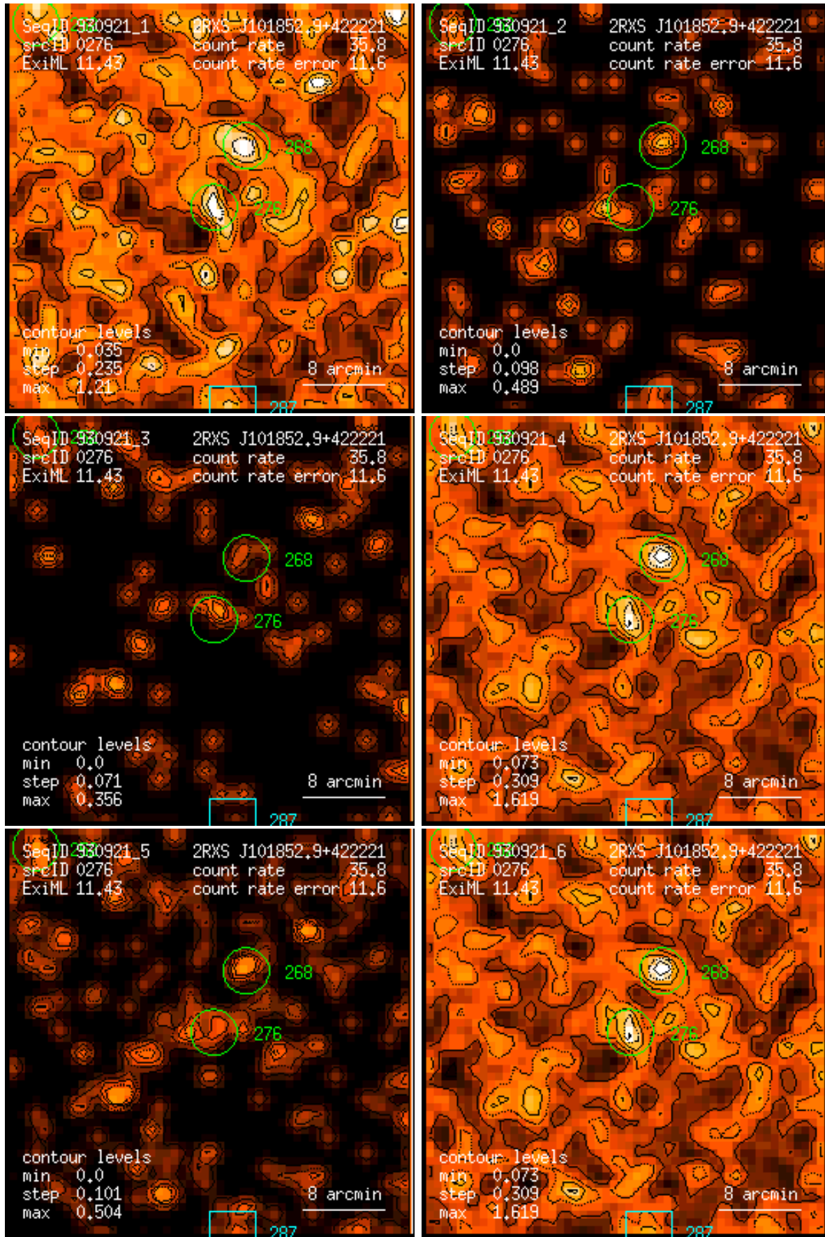
Figure 276: RASS 930921: detection 0276: band rate images, Gaussian filter: (1) PSPC channels 11 – 41, (2) 52 – 90, (3) 91 – 201, (4) 11 – 235, (5) 52 – 201, (6) 11 – 201. Broad band rates in counts/ks. Band rate contour levels in counts/ks/arcmin 2 .
