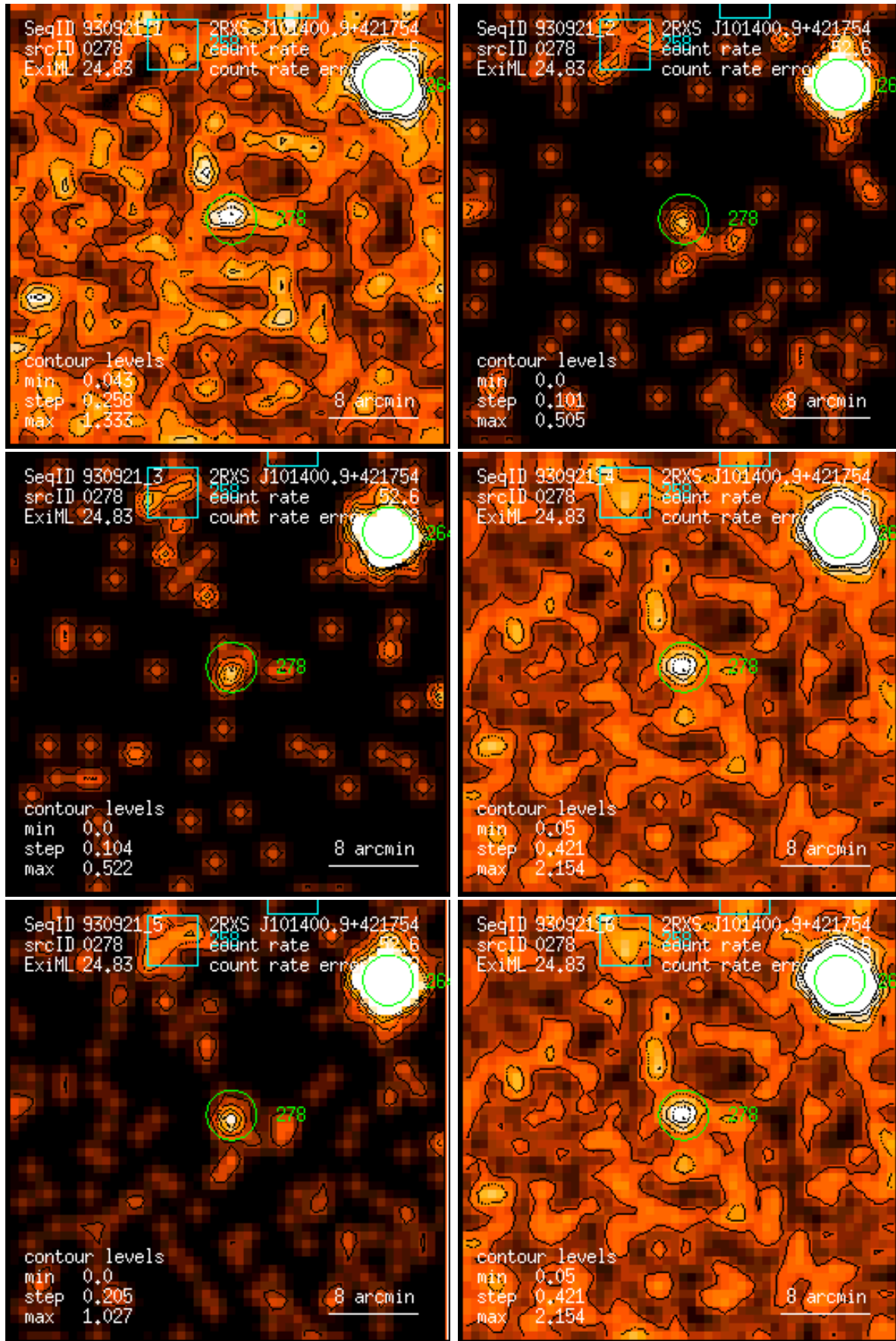
Figure 278: RASS 930921: detection 0278: band rate images, Gaussian filter: (1) PSPC channels 11 – 41, (2) 52 – 90, (3) 91 – 201, (4) 11 – 235, (5) 52 – 201, (6) 11 – 201. Broad band rates in counts/ks. Band rate contour levels in counts/ks/arcmin 2 .
