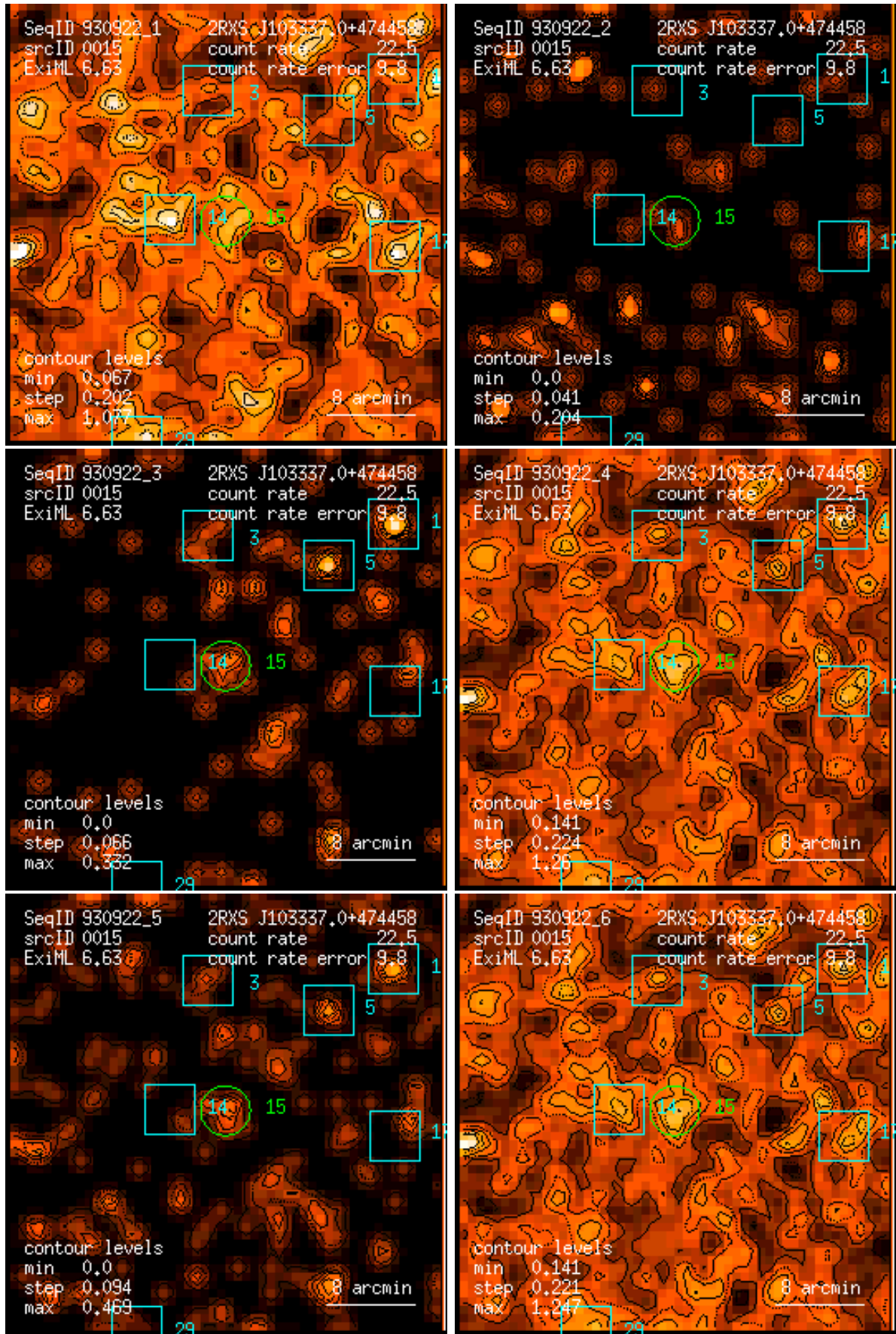
Figure 15: RASS 930922: detection 0015: band rate images, Gaussian filter: (1) PSPC channels 11 – 41, (2) 52 – 90, (3) 91 – 201, (4) 11 – 235, (5) 52 – 201, (6) 11 – 201. Broad band rates in counts/ks. Band rate contour levels in counts/ks/arcmin 2 .
