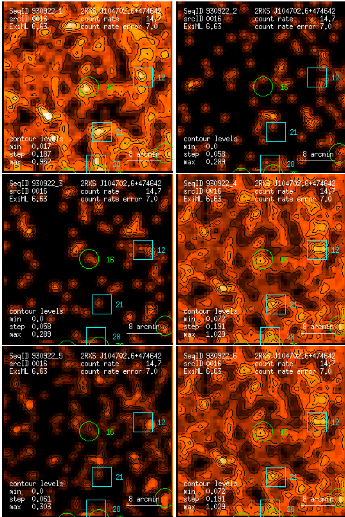
Figure 16: RASS 930922: detection 0016: band rate images, Gaussian filter: (1) PSPC channels 11 – 41, (2) 52 – 90, (3) 91 – 201, (4) 11 – 235, (5) 52 – 201, (6) 11 – 201. Broad band rates in counts/ks. Band rate contour levels in counts/ks/arcmin 2 .
