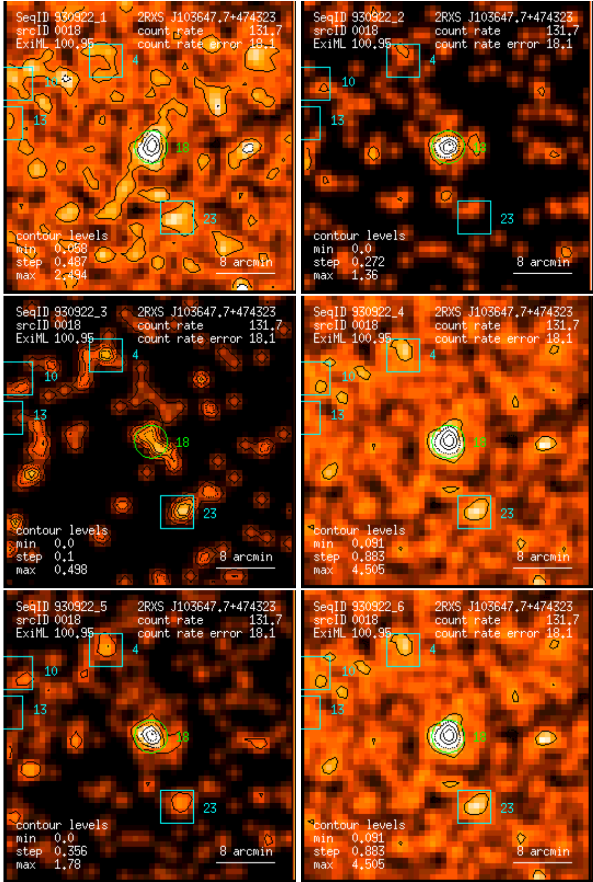
Figure 18: RASS 930922: detection 0018: band rate images, Gaussian filter: (1) PSPC channels 11 – 41, (2) 52 – 90, (3) 91 – 201, (4) 11 – 235, (5) 52 – 201, (6) 11 – 201. Broad band rates in counts/ks. Band rate contour levels in counts/ks/arcmin 2 .
