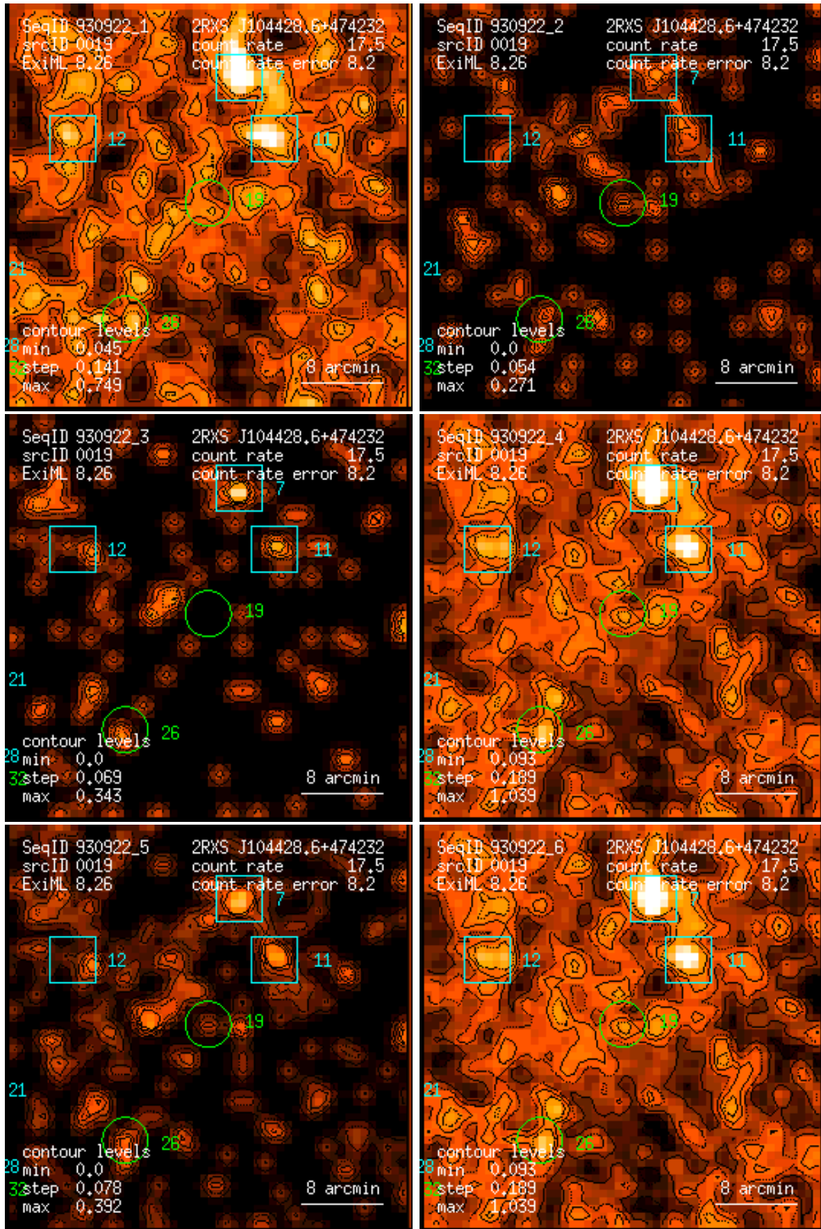
Figure 19: RASS 930922: detection 0019: band rate images, Gaussian filter: (1) PSPC channels 11 – 41, (2) 52 – 90, (3) 91 – 201, (4) 11 – 235, (5) 52 – 201, (6) 11 – 201. Broad band rates in counts/ks. Band rate contour levels in counts/ks/arcmin 2 .
