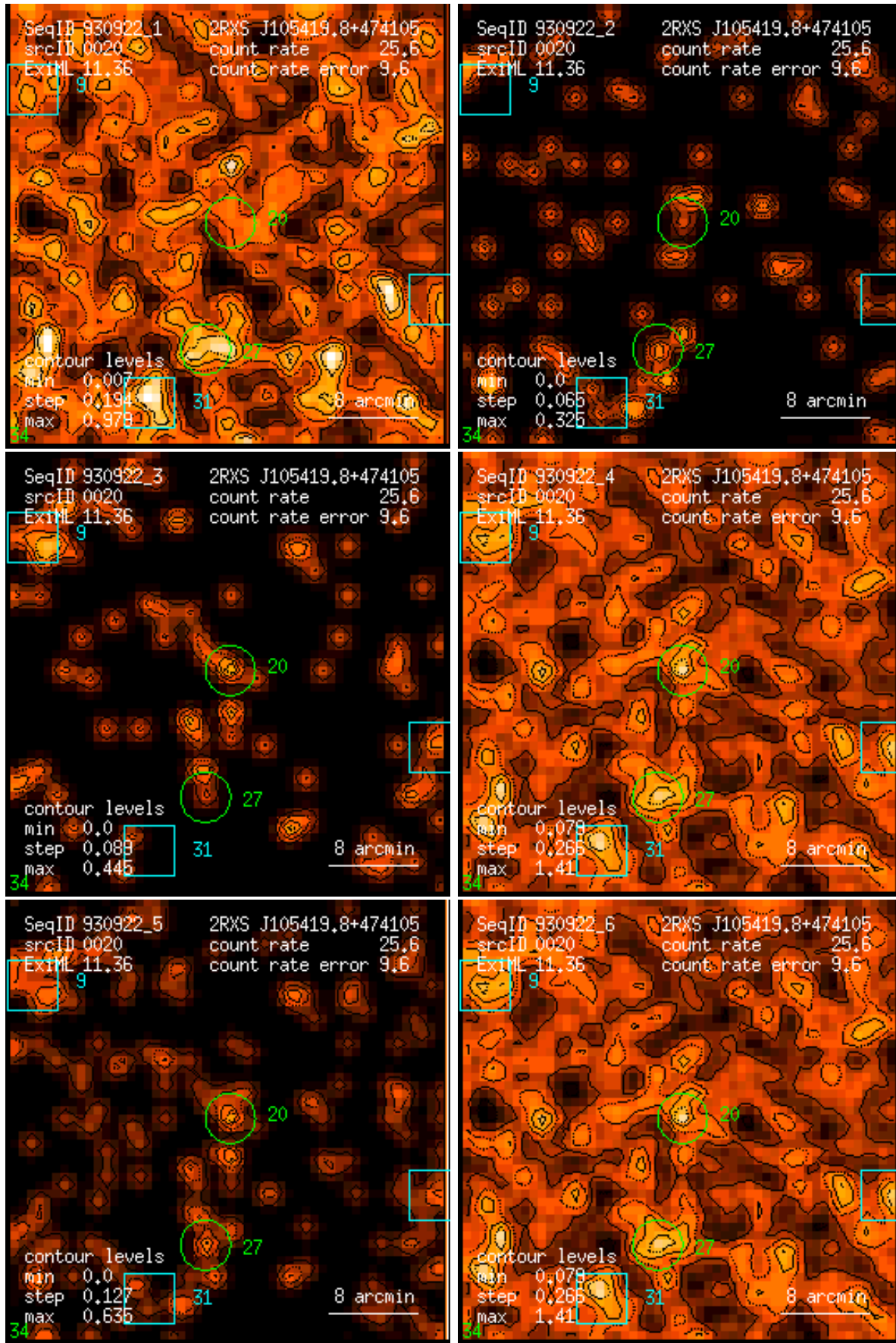
Figure 20: RASS 930922: detection 0020: band rate images, Gaussian filter: (1) PSPC channels 11 – 41, (2) 52 – 90, (3) 91 – 201, (4) 11 – 235, (5) 52 – 201, (6) 11 – 201. Broad band rates in counts/ks. Band rate contour levels in counts/ks/arcmin 2 .
