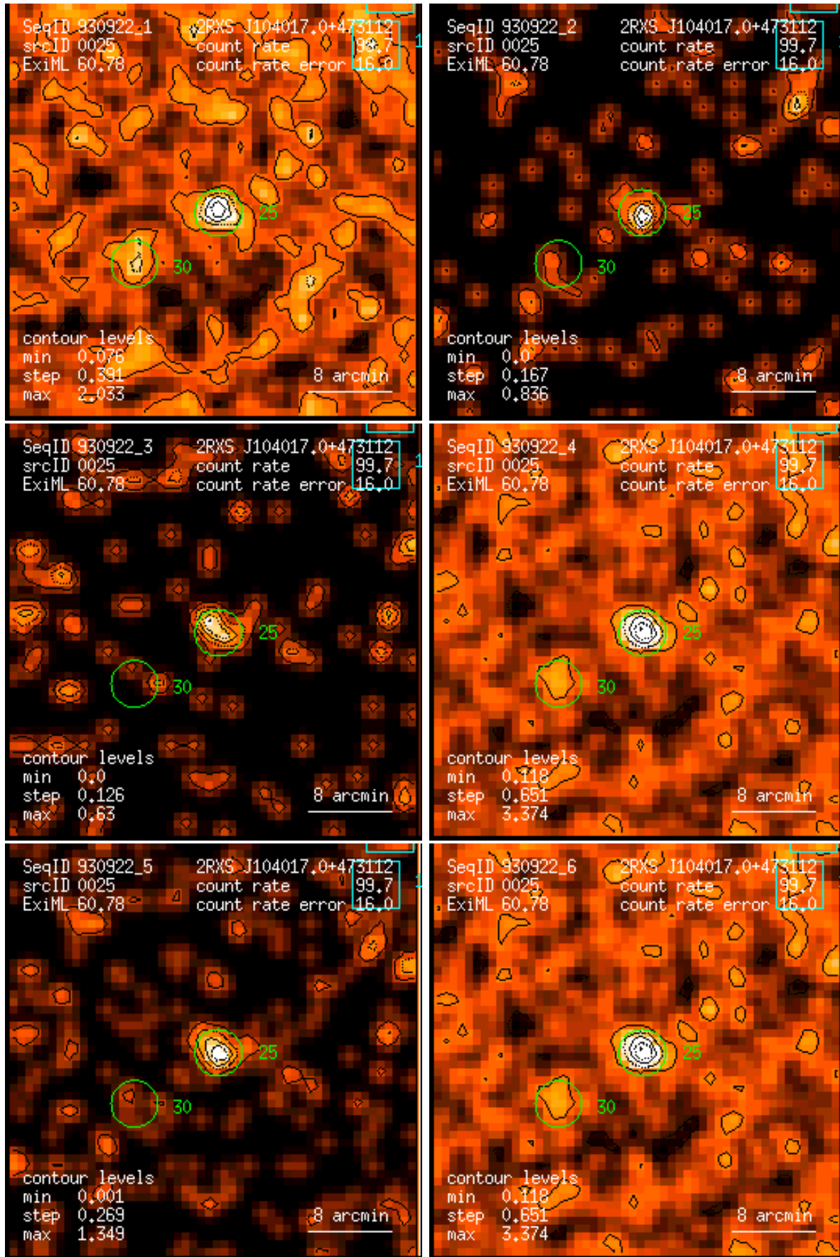
Figure 25: RASS 930922: detection 0025: band rate images, Gaussian filter: (1) PSPC channels 11 – 41, (2) 52 – 90, (3) 91 – 201, (4) 11 – 235, (5) 52 – 201, (6) 11 – 201. Broad band rates in counts/ks. Band rate contour levels in counts/ks/arcmin 2 .
