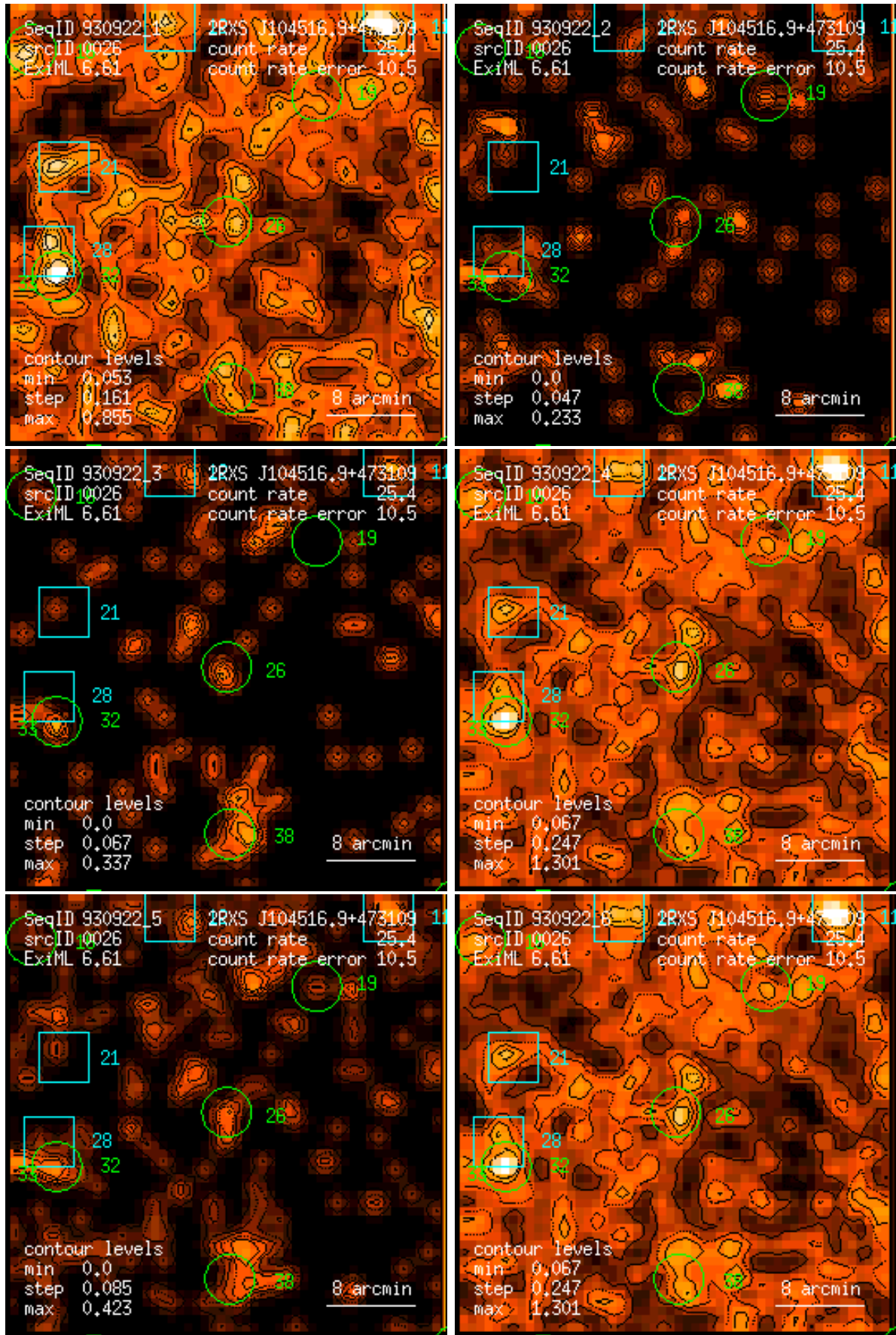
Figure 26: RASS 930922: detection 0026: band rate images, Gaussian filter: (1) PSPC channels 11 – 41, (2) 52 – 90, (3) 91 – 201, (4) 11 – 235, (5) 52 – 201, (6) 11 – 201. Broad band rates in counts/ks. Band rate contour levels in counts/ks/arcmin 2 .
