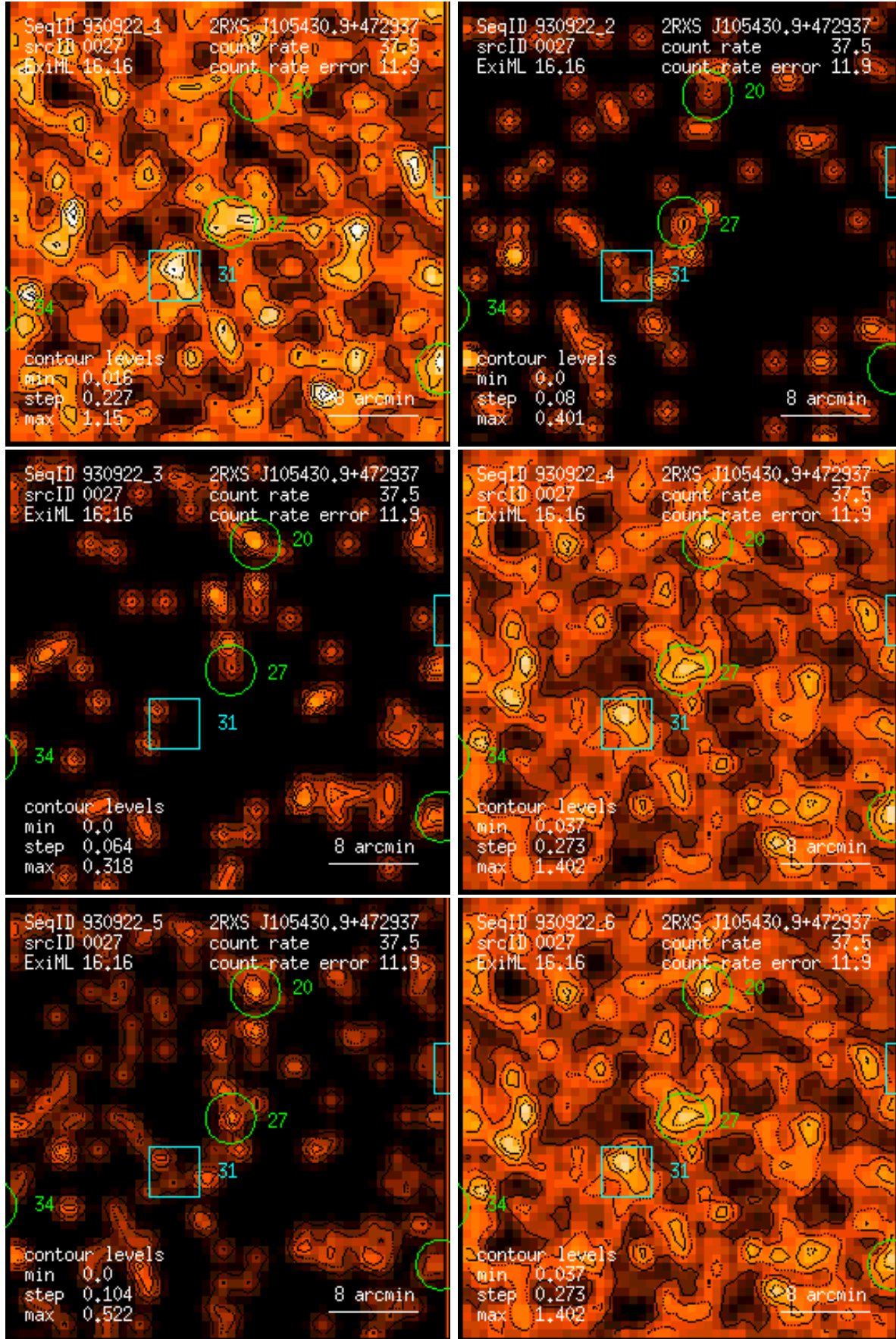
Figure 27: RASS 930922: detection 0027: band rate images, Gaussian filter: (1) PSPC channels 11 – 41, (2) 52 – 90, (3) 91 – 201, (4) 11 – 235, (5) 52 – 201, (6) 11 – 201. Broad band rates in counts/ks. Band rate contour levels in counts/ks/arcmin 2 .
