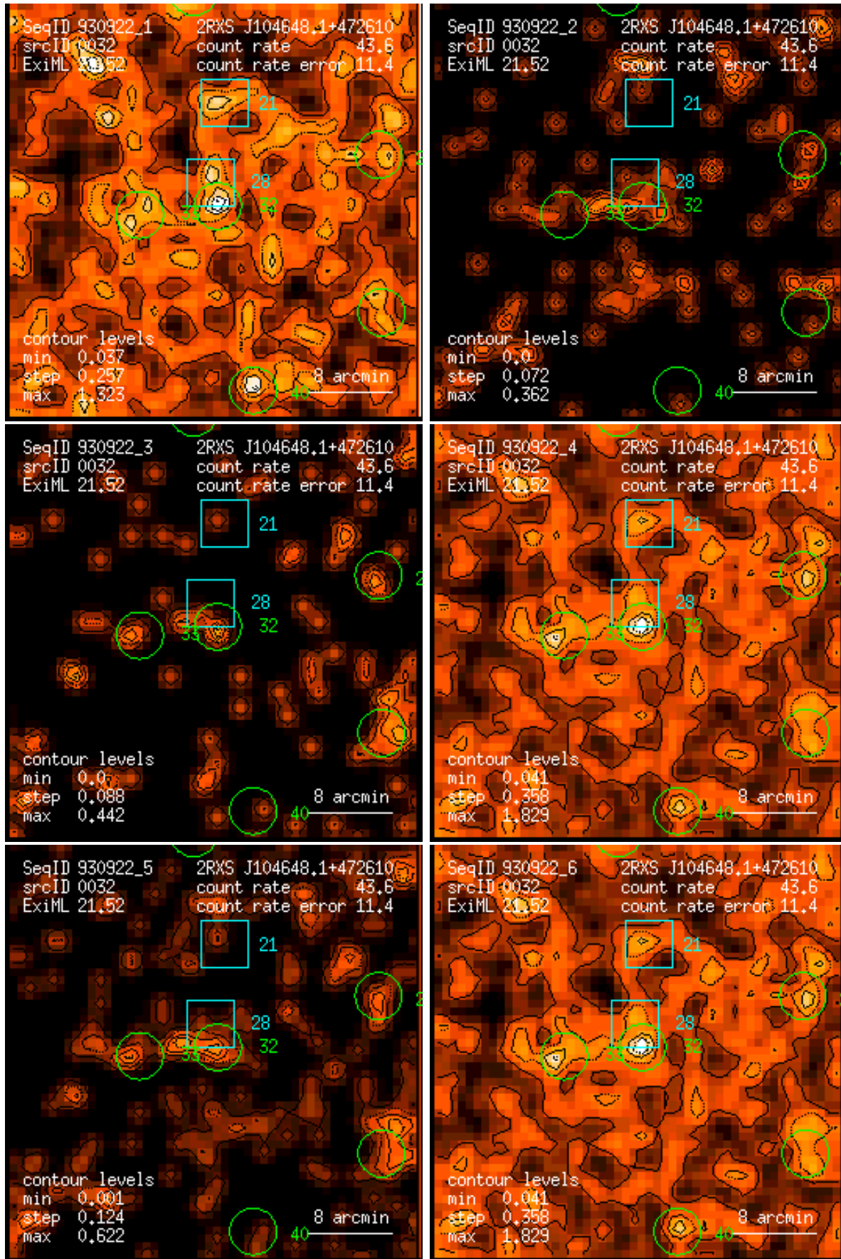
Figure 32: RASS 930922: detection 0032: band rate images, Gaussian filter: (1) PSPC channels 11 – 41, (2) 52 – 90, (3) 91 – 201, (4) 11 – 235, (5) 52 – 201, (6) 11 – 201. Broad band rates in counts/ks. Band rate contour levels in counts/ks/arcmin 2 .
