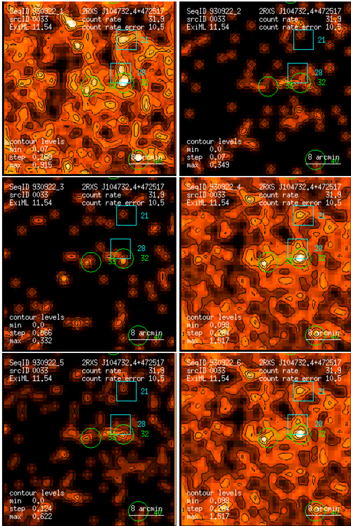
Figure 33: RASS 930922: detection 0033: band rate images, Gaussian filter: (1) PSPC channels 11 – 41, (2) 52 – 90, (3) 91 – 201, (4) 11 – 235, (5) 52 – 201, (6) 11 – 201. Broad band rates in counts/ks. Band rate contour levels in counts/ks/arcmin 2 .
