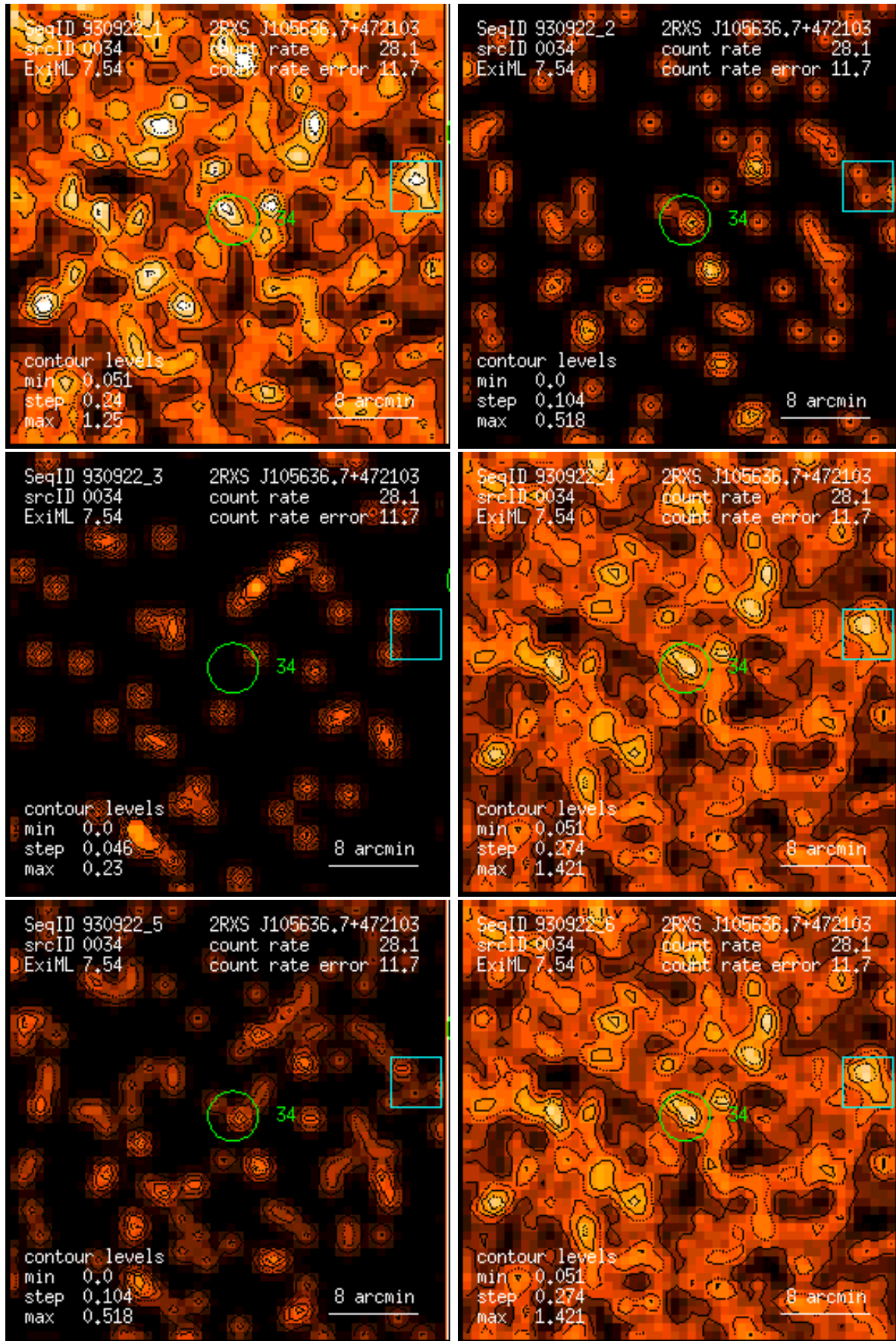
Figure 34: RASS 930922: detection 0034: band rate images, Gaussian filter: (1) PSPC channels 11 – 41, (2) 52 – 90, (3) 91 – 201, (4) 11 – 235, (5) 52 – 201, (6) 11 – 201. Broad band rates in counts/ks. Band rate contour levels in counts/ks/arcmin 2 .
