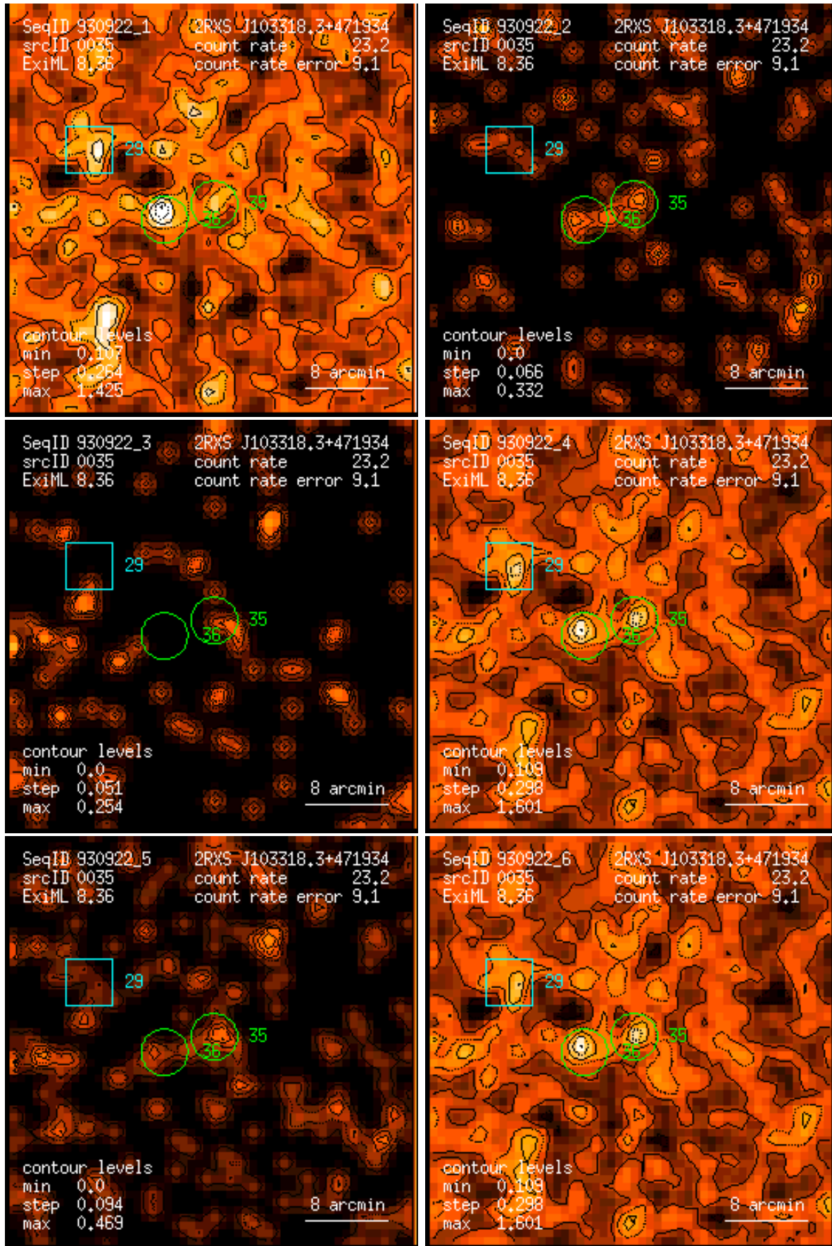
Figure 35: RASS 930922: detection 0035: band rate images, Gaussian filter: (1) PSPC channels 11 – 41, (2) 52 – 90, (3) 91 – 201, (4) 11 – 235, (5) 52 – 201, (6) 11 – 201. Broad band rates in counts/ks. Band rate contour levels in counts/ks/arcmin 2 .
