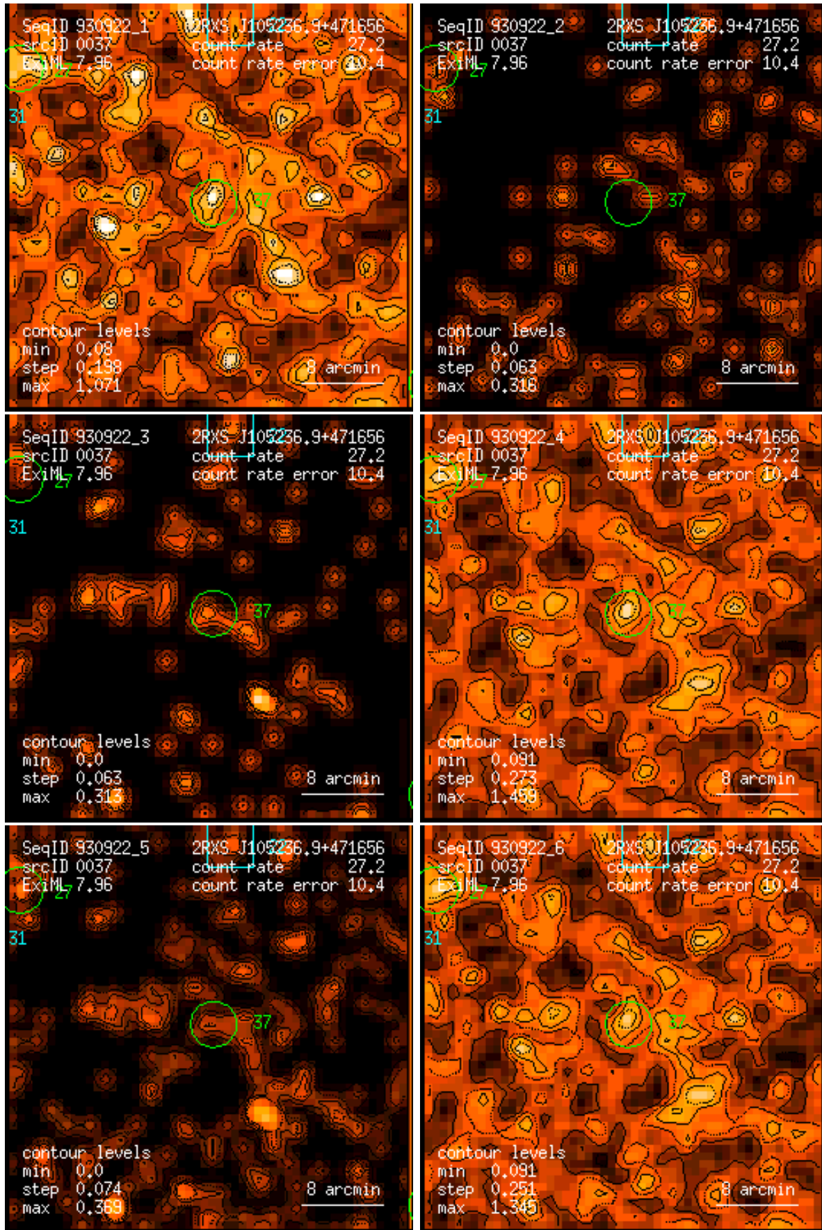
Figure 37: RASS 930922: detection 0037: band rate images, Gaussian filter: (1) PSPC channels 11 – 41, (2) 52 – 90, (3) 91 – 201, (4) 11 – 235, (5) 52 – 201, (6) 11 – 201. Broad band rates in counts/ks. Band rate contour levels in counts/ks/arcmin 2 .
