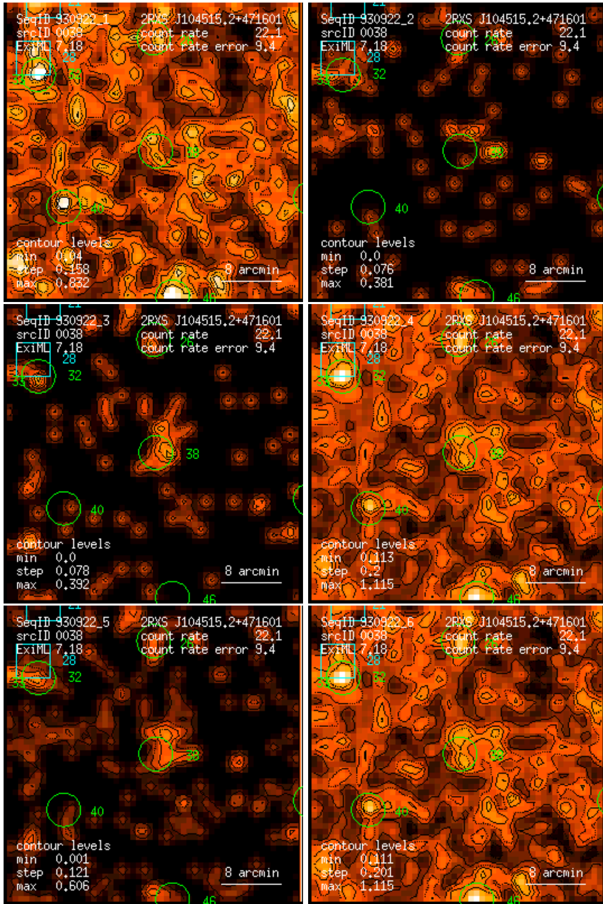
Figure 38: RASS 930922: detection 0038: band rate images, Gaussian filter: (1) PSPC channels 11 – 41, (2) 52 – 90, (3) 91 – 201, (4) 11 – 235, (5) 52 – 201, (6) 11 – 201. Broad band rates in counts/ks. Band rate contour levels in counts/ks/arcmin 2 .
