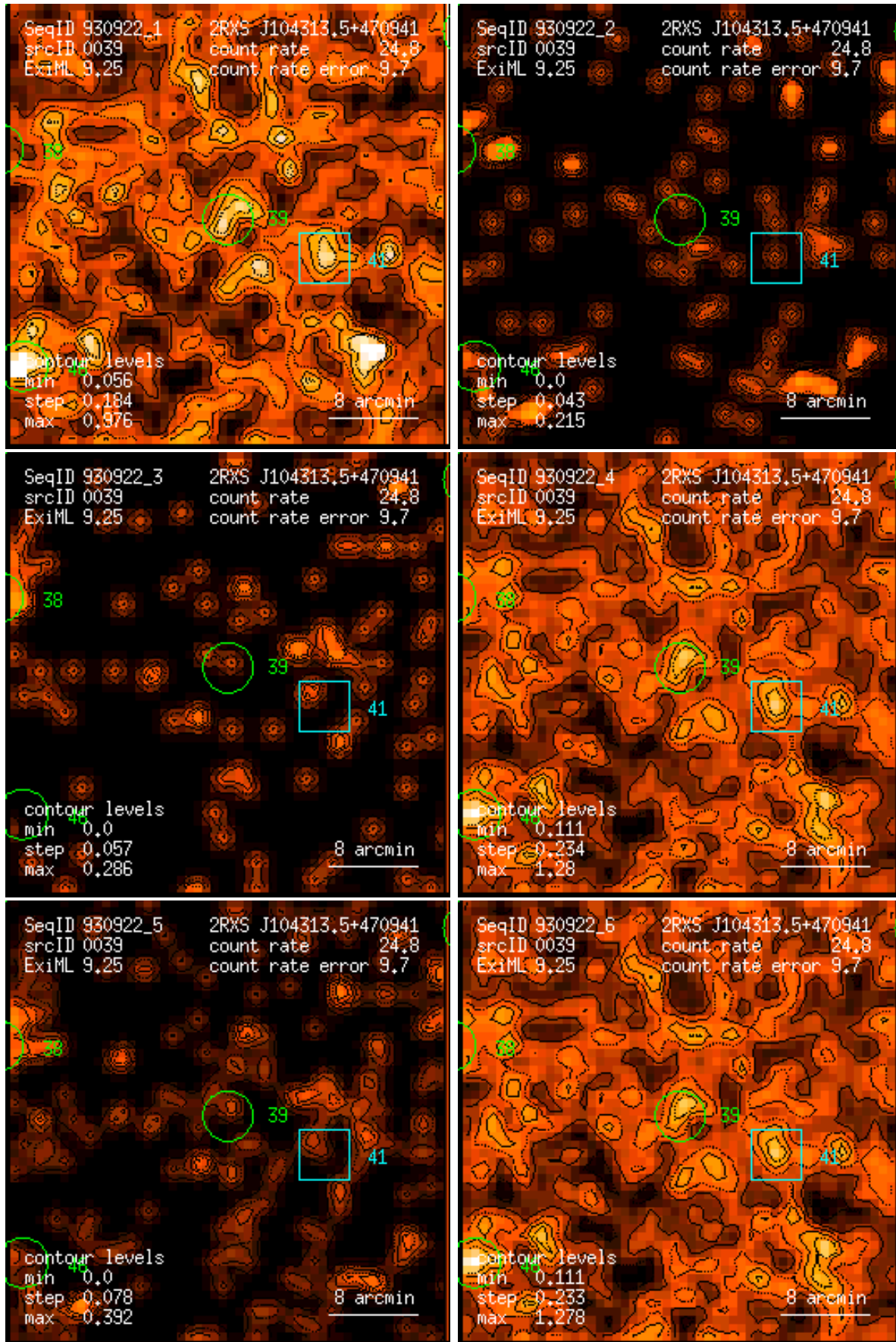
Figure 39: RASS 930922: detection 0039: band rate images, Gaussian filter: (1) PSPC channels 11 – 41, (2) 52 – 90, (3) 91 – 201, (4) 11 – 235, (5) 52 – 201, (6) 11 – 201. Broad band rates in counts/ks. Band rate contour levels in counts/ks/arcmin 2 .
