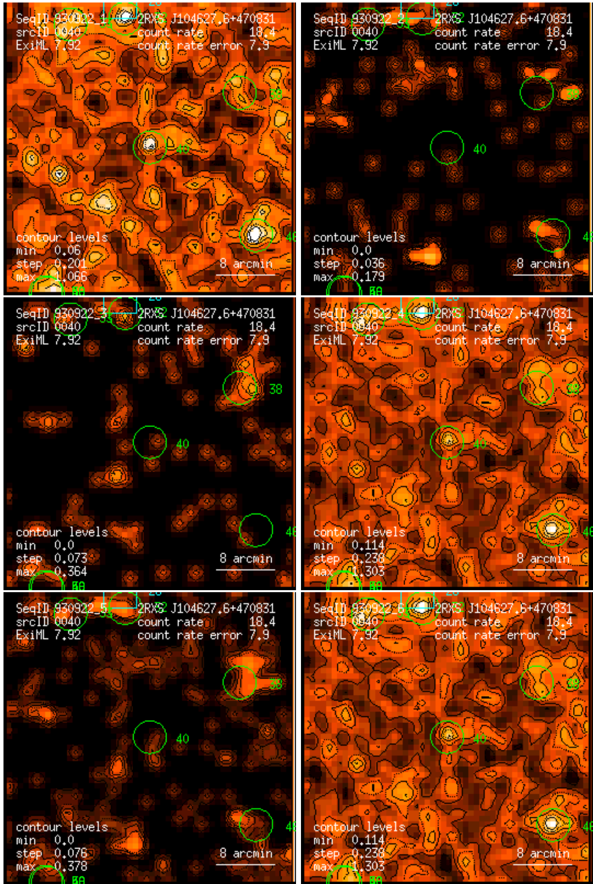
Figure 40: RASS 930922: detection 0040: band rate images, Gaussian filter: (1) PSPC channels 11 – 41, (2) 52 – 90, (3) 91 – 201, (4) 11 – 235, (5) 52 – 201, (6) 11 – 201. Broad band rates in counts/ks. Band rate contour levels in counts/ks/arcmin 2 .
