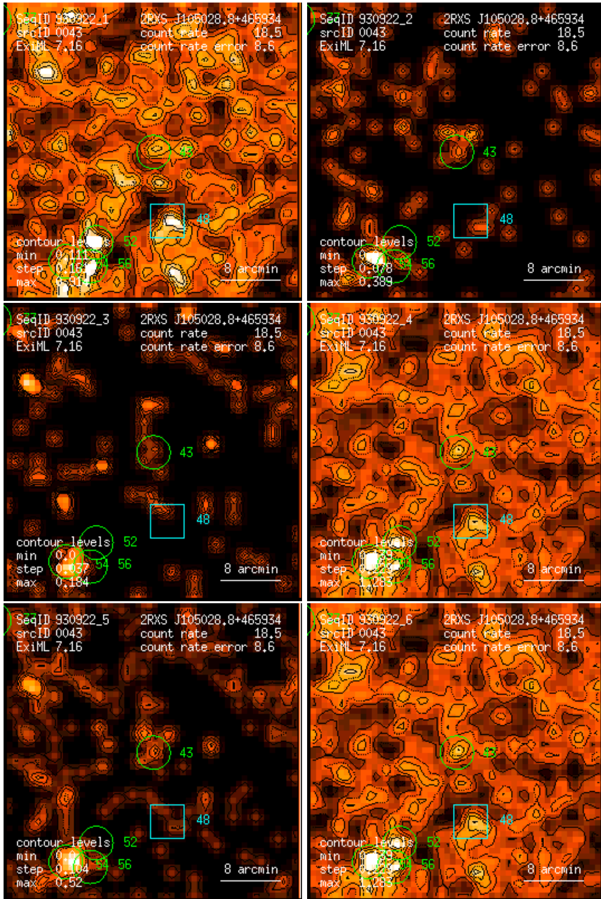
Figure 43: RASS 930922: detection 0043: band rate images, Gaussian filter: (1) PSPC channels 11 – 41, (2) 52 – 90, (3) 91 – 201, (4) 11 – 235, (5) 52 – 201, (6) 11 – 201. Broad band rates in counts/ks. Band rate contour levels in counts/ks/arcmin 2 .
