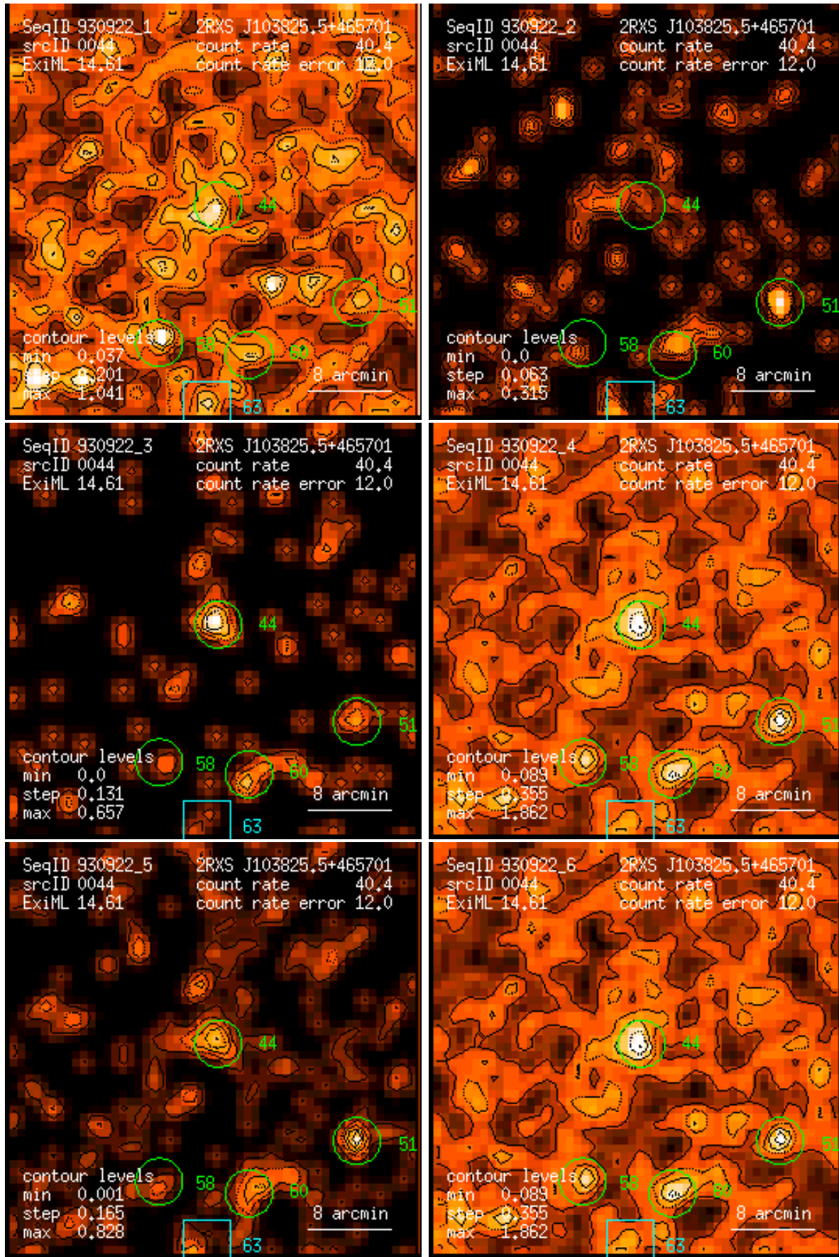
Figure 44: RASS 930922: detection 0044: band rate images, Gaussian filter: (1) PSPC channels 11 – 41, (2) 52 – 90, (3) 91 – 201, (4) 11 – 235, (5) 52 – 201, (6) 11 – 201. Broad band rates in counts/ks. Band rate contour levels in counts/ks/arcmin 2 .
