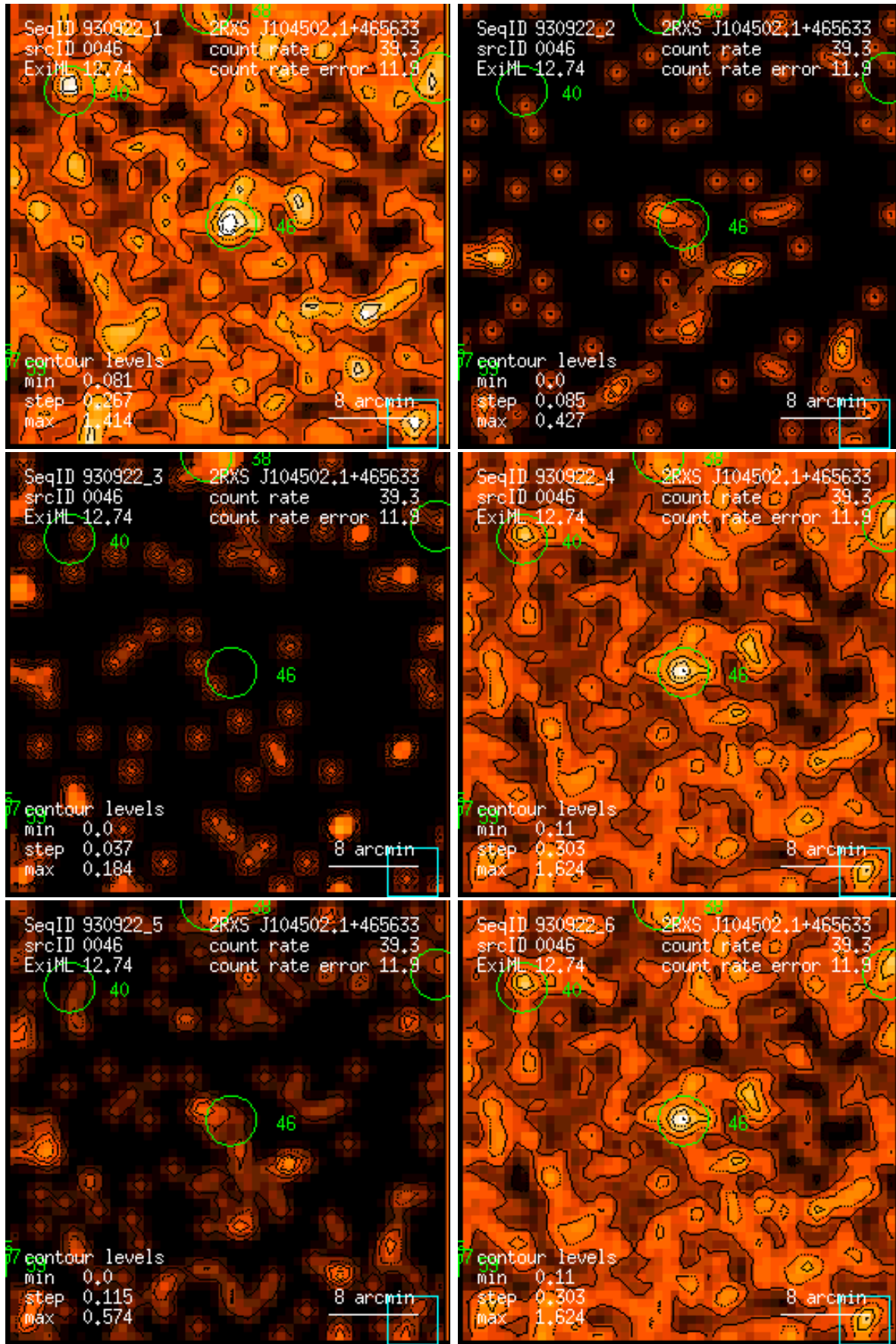
Figure 46: RASS 930922: detection 0046: band rate images, Gaussian filter: (1) PSPC channels 11 – 41, (2) 52 – 90, (3) 91 – 201, (4) 11 – 235, (5) 52 – 201, (6) 11 – 201. Broad band rates in counts/ks. Band rate contour levels in counts/ks/arcmin 2 .
