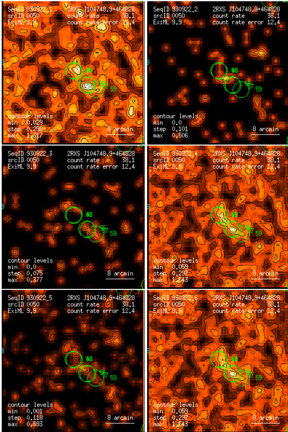
Figure 50: RASS 930922: detection 0050: band rate images, Gaussian filter: (1) PSPC channels 11 – 41, (2) 52 – 90, (3) 91 – 201, (4) 11 – 235, (5) 52 – 201, (6) 11 – 201. Broad band rates in counts/ks. Band rate contour levels in counts/ks/arcmin 2 .
