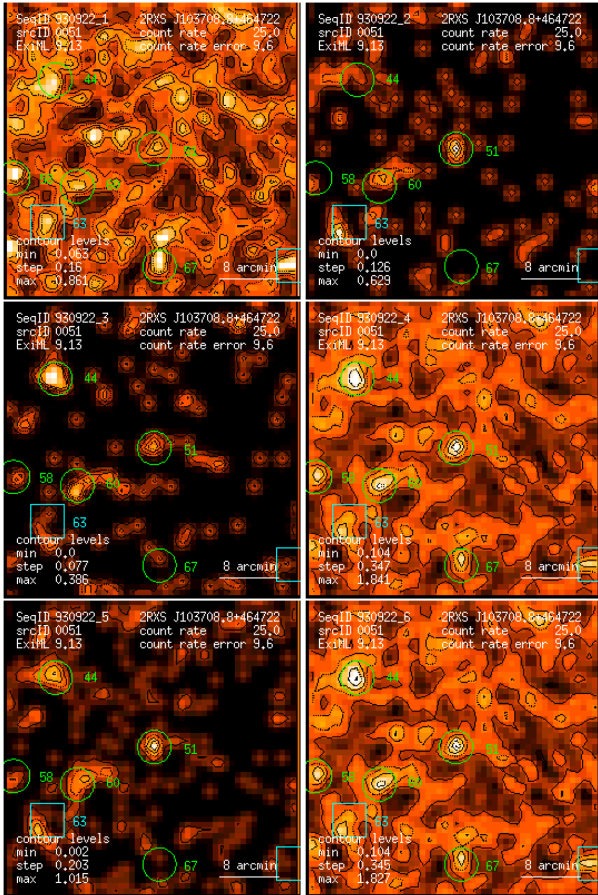
Figure 51: RASS 930922: detection 0051: band rate images, Gaussian filter: (1) PSPC channels 11 – 41, (2) 52 – 90, (3) 91 – 201, (4) 11 – 235, (5) 52 – 201, (6) 11 – 201. Broad band rates in counts/ks. Band rate contour levels in counts/ks/arcmin 2 .
