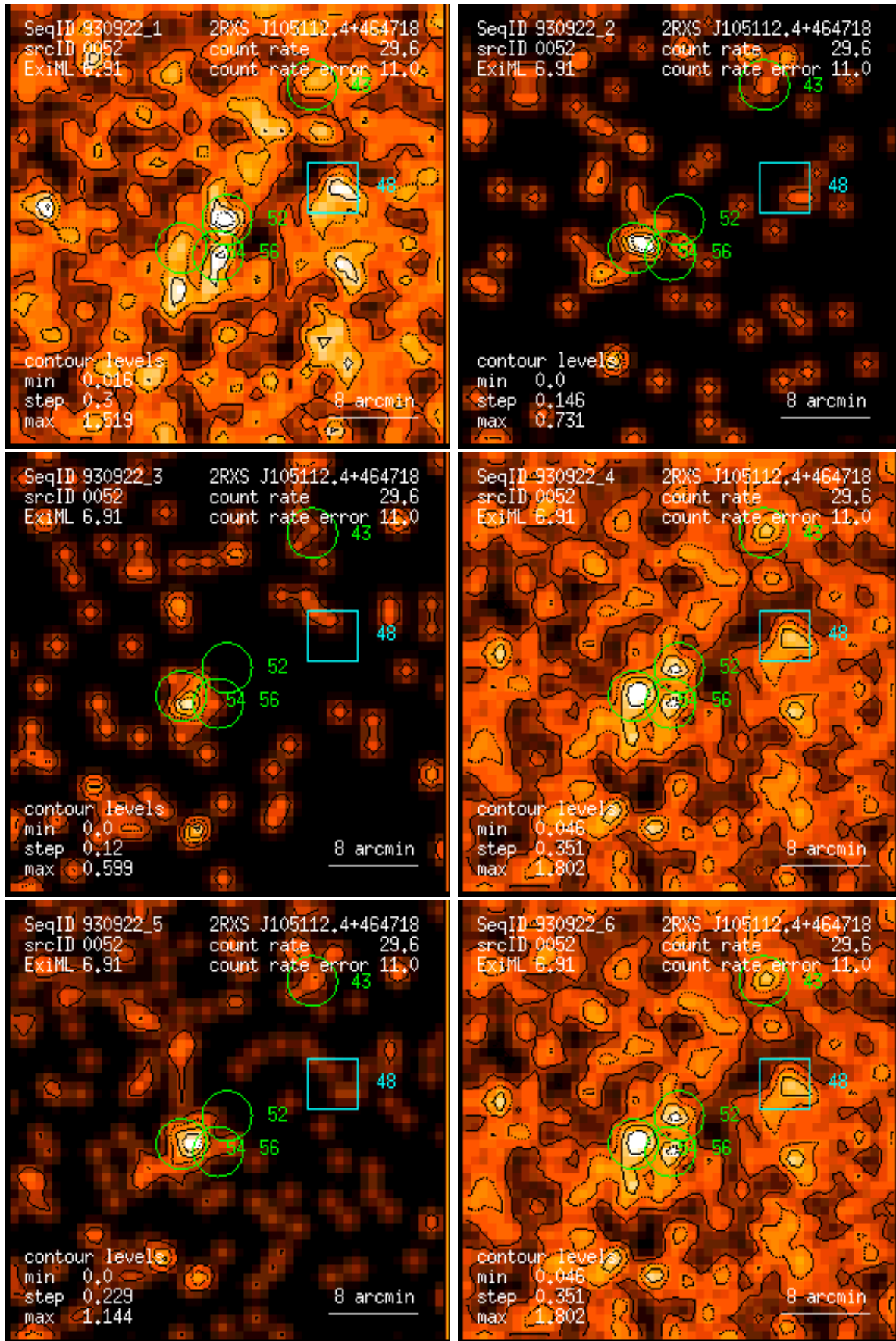
Figure 52: RASS 930922: detection 0052: band rate images, Gaussian filter: (1) PSPC channels 11 – 41, (2) 52 – 90, (3) 91 – 201, (4) 11 – 235, (5) 52 – 201, (6) 11 – 201. Broad band rates in counts/ks. Band rate contour levels in counts/ks/arcmin 2 .
