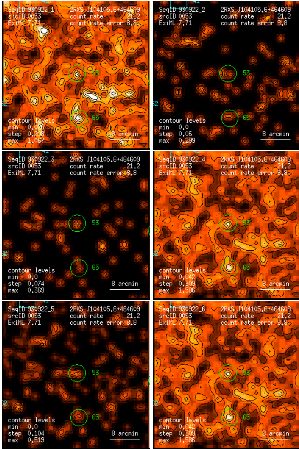
Figure 53: RASS 930922: detection 0053: band rate images, Gaussian filter: (1) PSPC channels 11 – 41, (2) 52 – 90, (3) 91 – 201, (4) 11 – 235, (5) 52 – 201, (6) 11 – 201. Broad band rates in counts/ks. Band rate contour levels in counts/ks/arcmin 2 .
