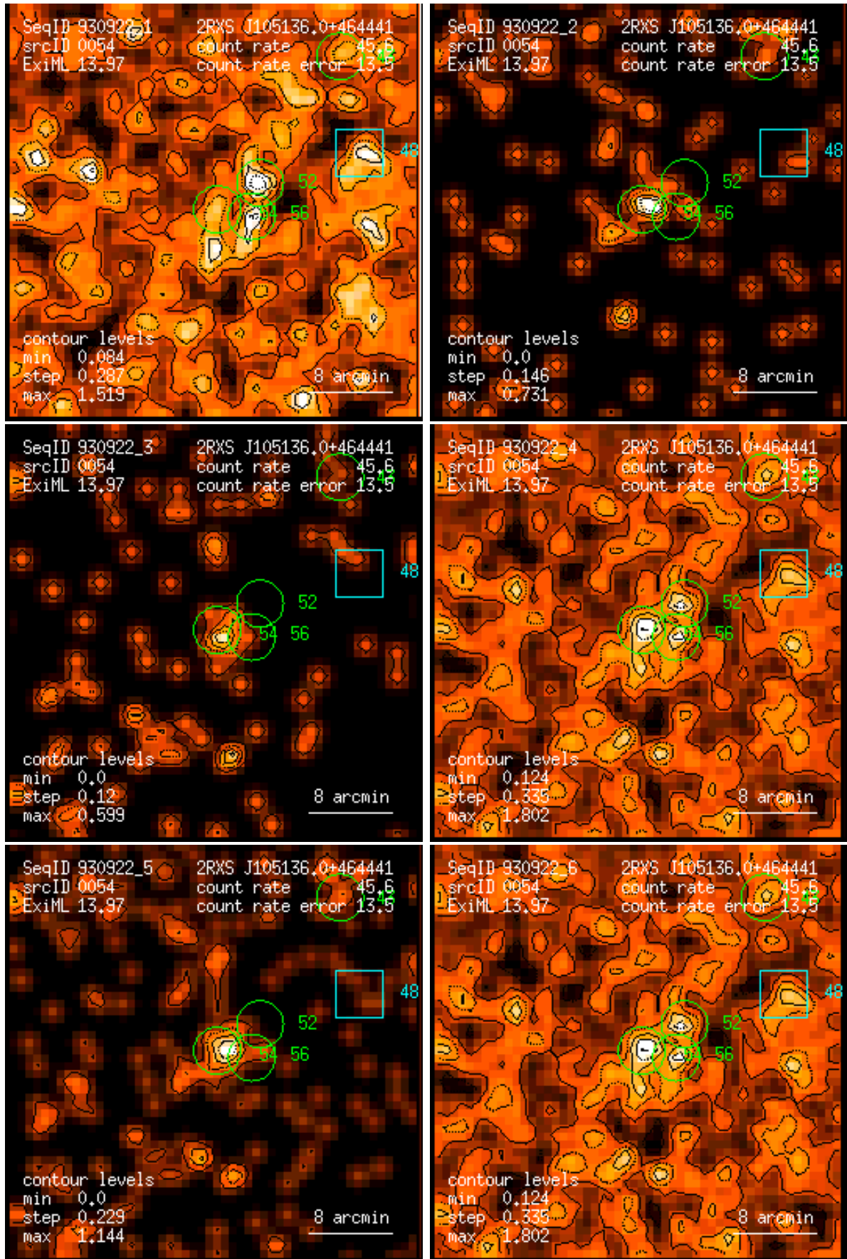
Figure 54: RASS 930922: detection 0054: band rate images, Gaussian filter: (1) PSPC channels 11 – 41, (2) 52 – 90, (3) 91 – 201, (4) 11 – 235, (5) 52 – 201, (6) 11 – 201. Broad band rates in counts/ks. Band rate contour levels in counts/ks/arcmin 2 .
