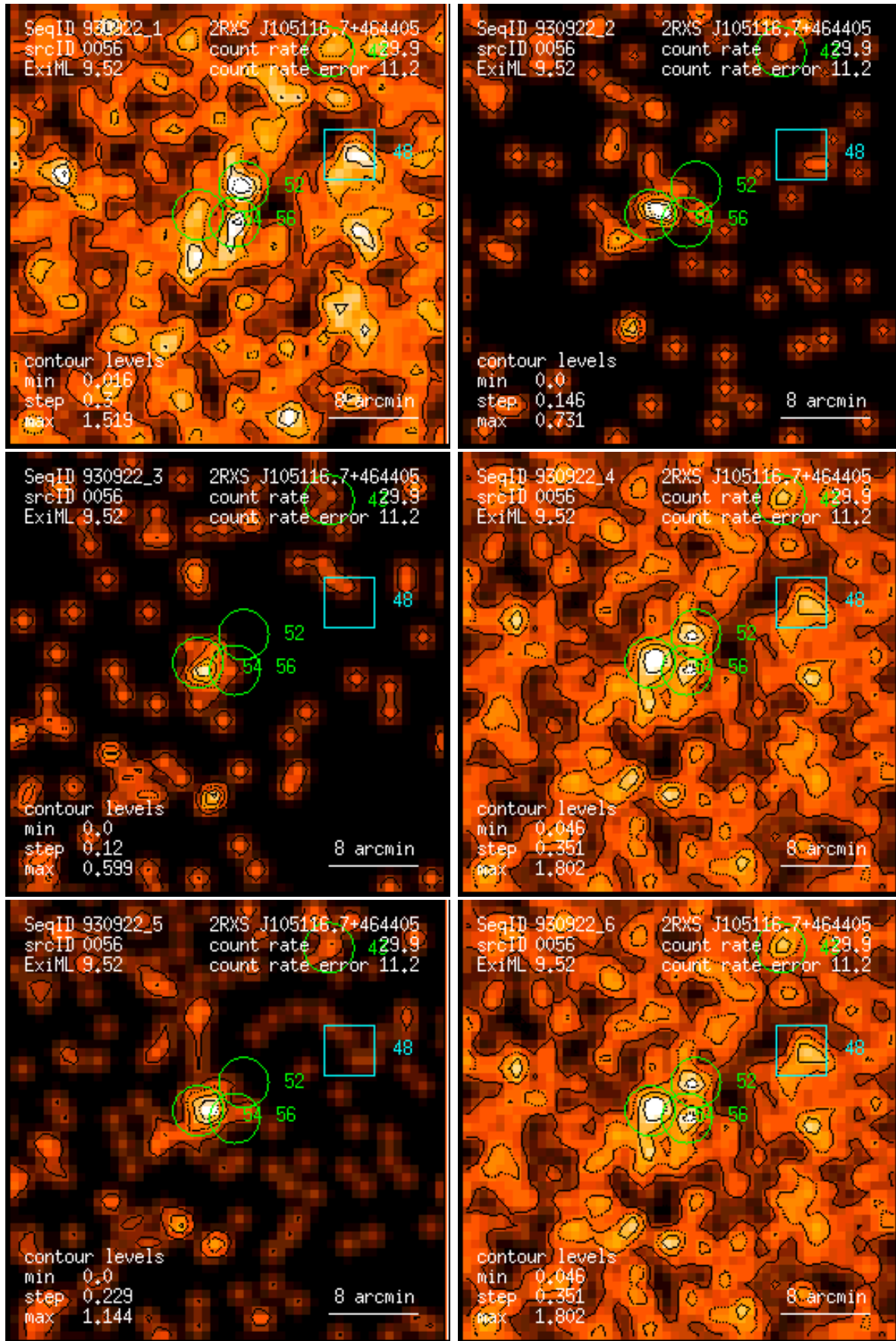
Figure 56: RASS 930922: detection 0056: band rate images, Gaussian filter: (1) PSPC channels 11 – 41, (2) 52 – 90, (3) 91 – 201, (4) 11 – 235, (5) 52 – 201, (6) 11 – 201. Broad band rates in counts/ks. Band rate contour levels in counts/ks/arcmin 2 .
