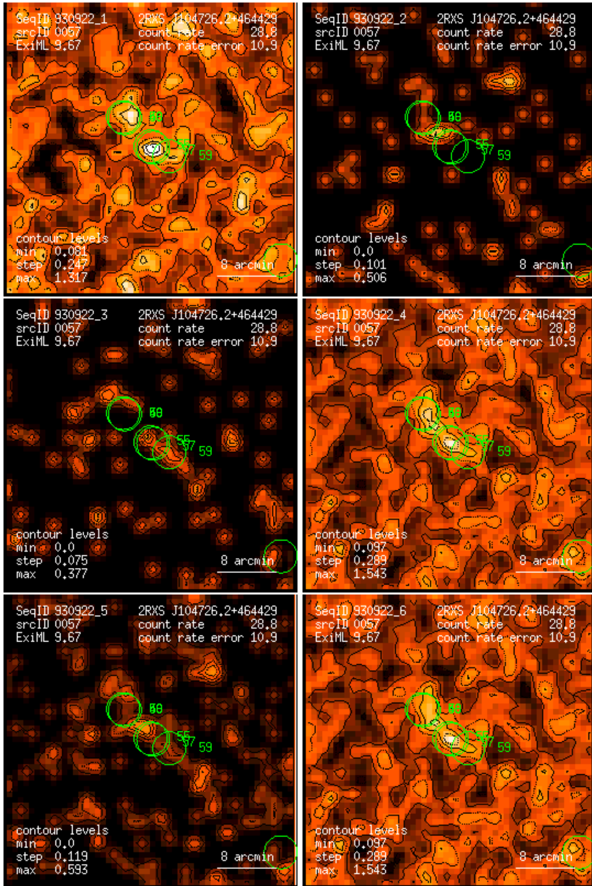
Figure 57: RASS 930922: detection 0057: band rate images, Gaussian filter: (1) PSPC channels 11 – 41, (2) 52 – 90, (3) 91 – 201, (4) 11 – 235, (5) 52 – 201, (6) 11 – 201. Broad band rates in counts/ks. Band rate contour levels in counts/ks/arcmin 2 .
