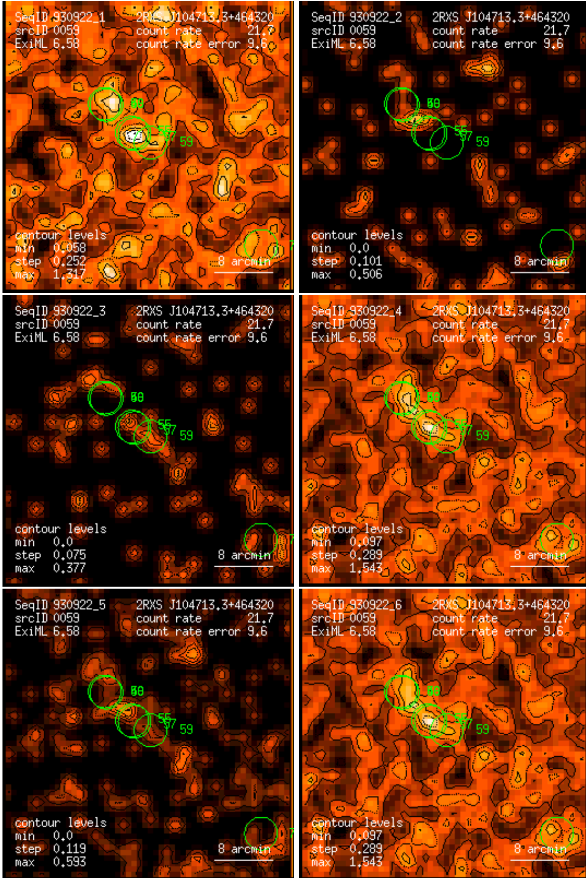
Figure 59: RASS 930922: detection 0059: band rate images, Gaussian filter: (1) PSPC channels 11 – 41, (2) 52 – 90, (3) 91 – 201, (4) 11 – 235, (5) 52 – 201, (6) 11 – 201. Broad band rates in counts/ks. Band rate contour levels in counts/ks/arcmin 2 .
