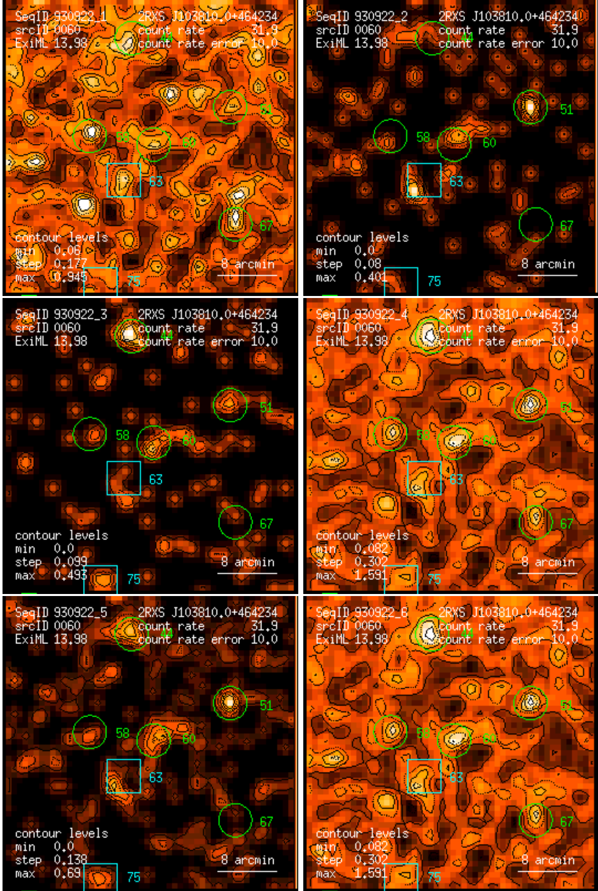
Figure 60: RASS 930922: detection 0060: band rate images, Gaussian filter: (1) PSPC channels 11 – 41, (2) 52 – 90, (3) 91 – 201, (4) 11 – 235, (5) 52 – 201, (6) 11 – 201. Broad band rates in counts/ks. Band rate contour levels in counts/ks/arcmin 2 .
