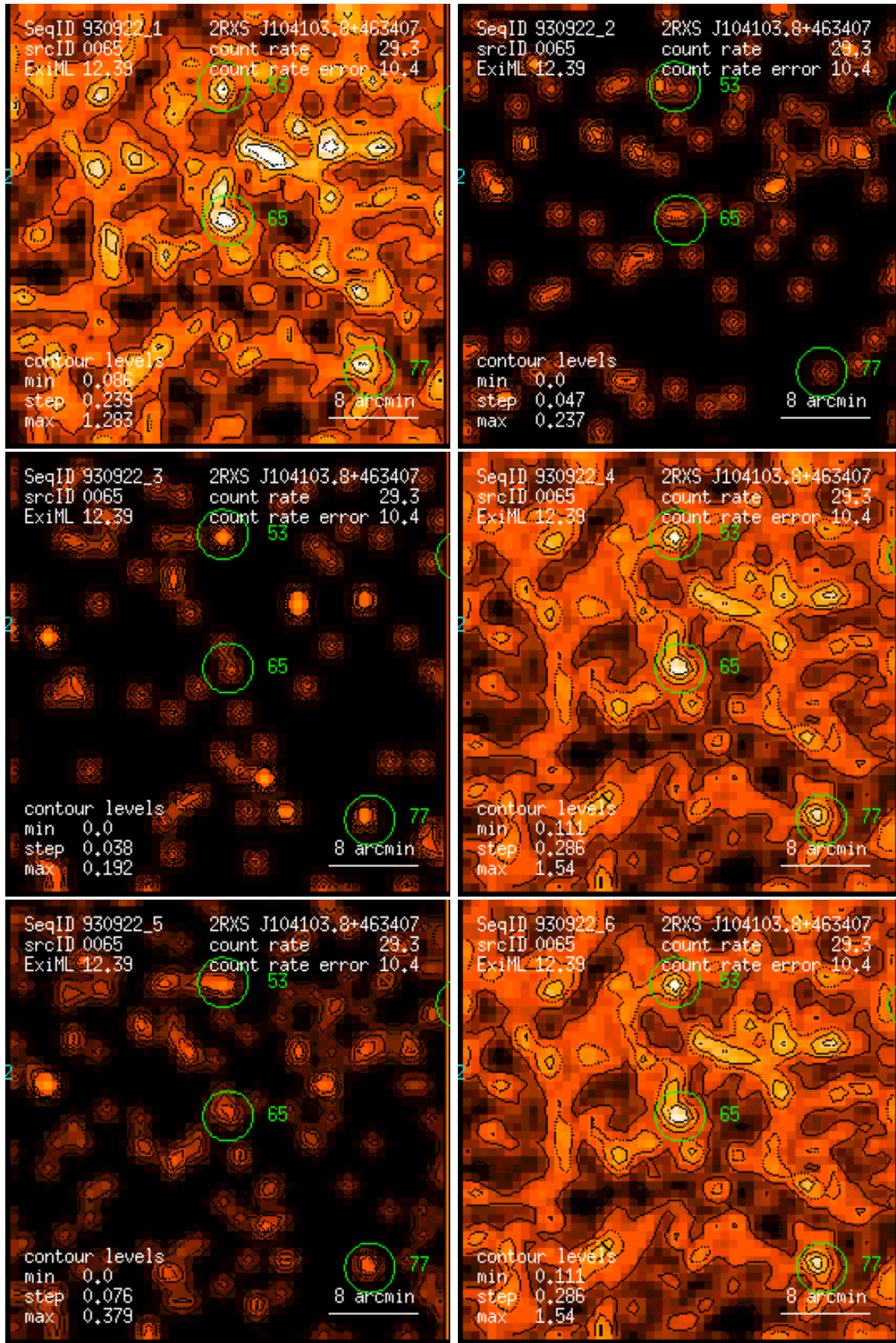
Figure 65: RASS 930922: detection 0065: band rate images, Gaussian filter: (1) PSPC channels 11 – 41, (2) 52 – 90, (3) 91 – 201, (4) 11 – 235, (5) 52 – 201, (6) 11 – 201. Broad band rates in counts/ks. Band rate contour levels in counts/ks/arcmin 2 .
