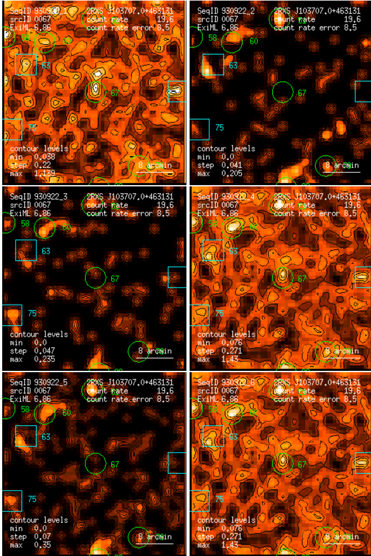
Figure 67: RASS 930922: detection 0067: band rate images, Gaussian filter: (1) PSPC channels 11 – 41, (2) 52 – 90, (3) 91 – 201, (4) 11 – 235, (5) 52 – 201, (6) 11 – 201. Broad band rates in counts/ks. Band rate contour levels in counts/ks/arcmin 2 .
