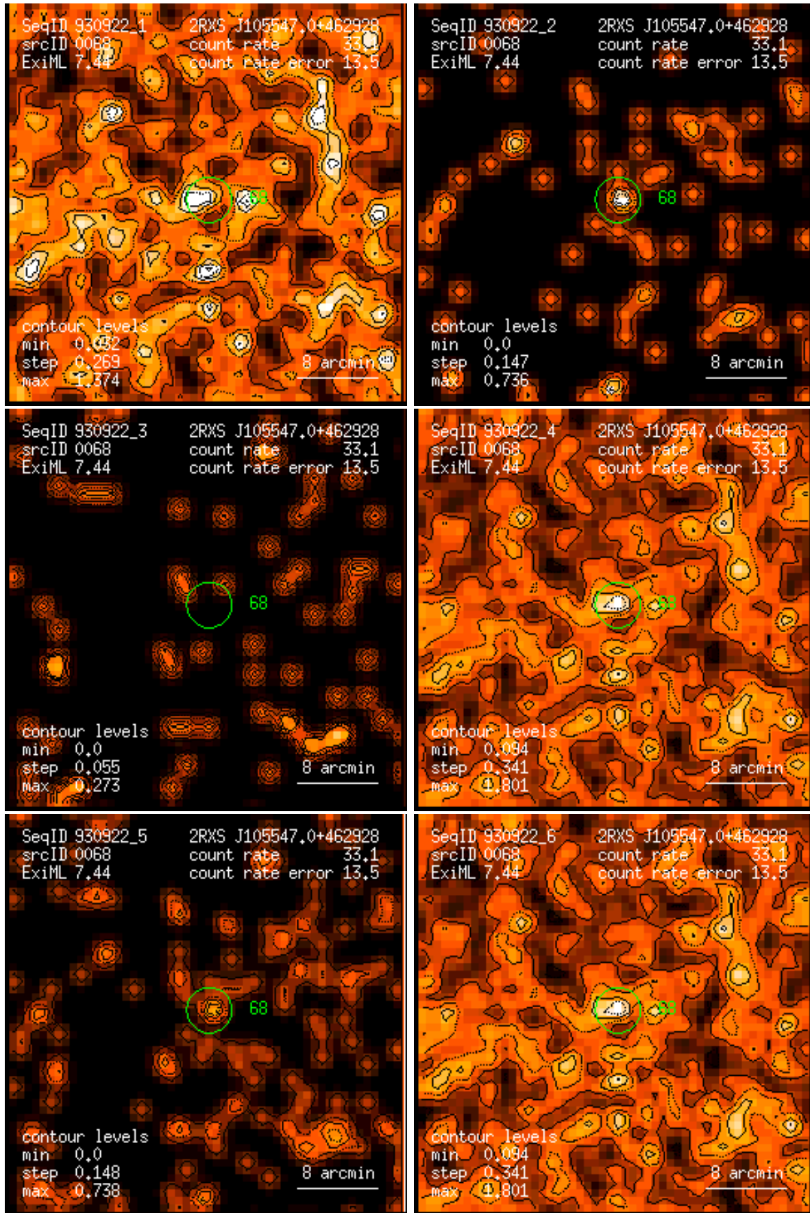
Figure 68: RASS 930922: detection 0068: band rate images, Gaussian filter: (1) PSPC channels 11 – 41, (2) 52 – 90, (3) 91 – 201, (4) 11 – 235, (5) 52 – 201, (6) 11 – 201. Broad band rates in counts/ks. Band rate contour levels in counts/ks/arcmin 2 .
