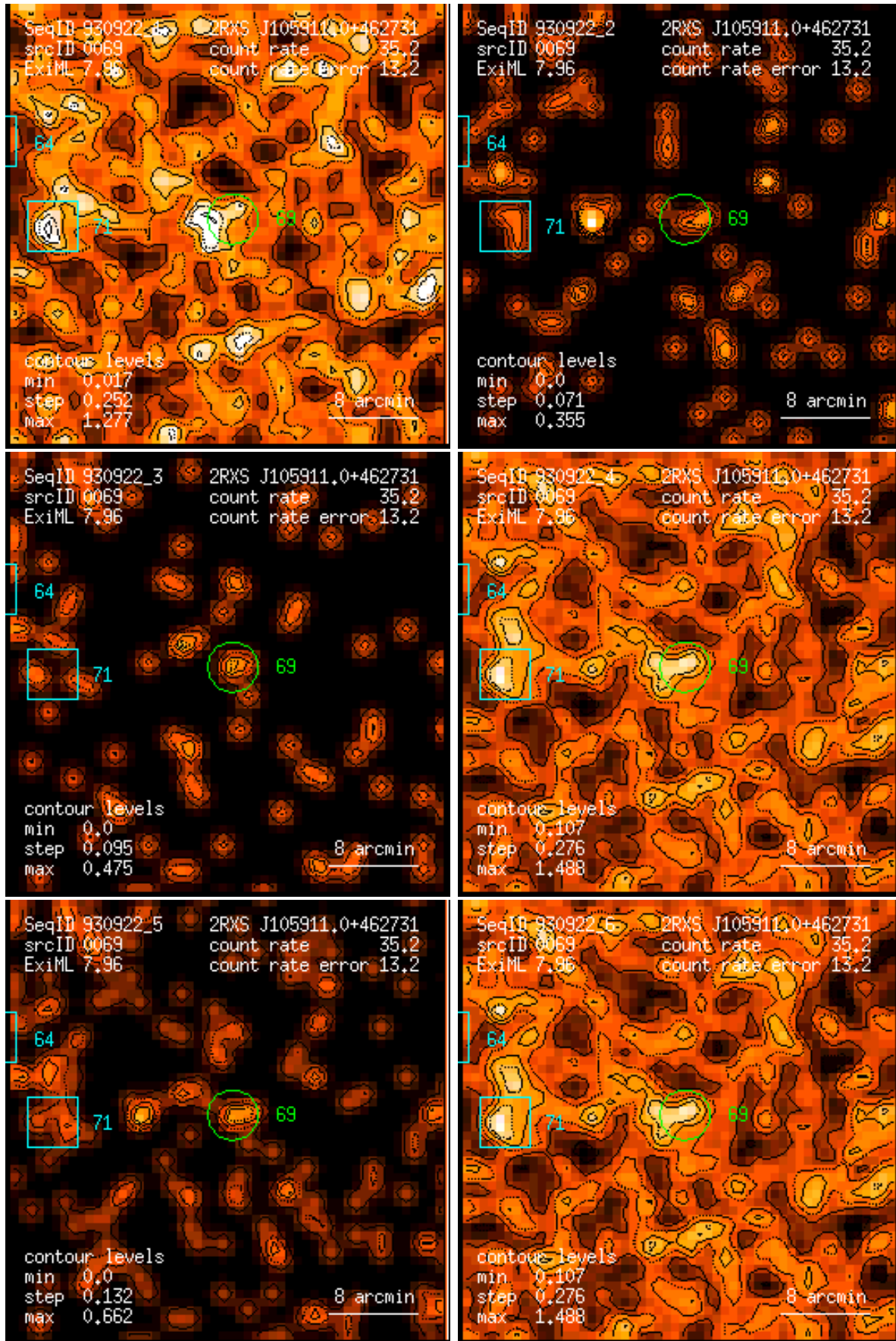
Figure 69: RASS 930922: detection 0069: band rate images, Gaussian filter: (1) PSPC channels 11 – 41, (2) 52 – 90, (3) 91 – 201, (4) 11 – 235, (5) 52 – 201, (6) 11 – 201. Broad band rates in counts/ks. Band rate contour levels in counts/ks/arcmin 2 .
