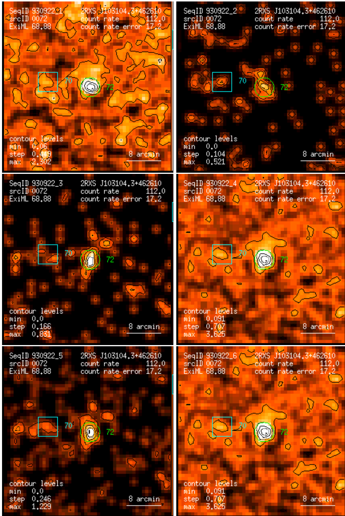
Figure 72: RASS 930922: detection 0072: band rate images, Gaussian filter: (1) PSPC channels 11 – 41, (2) 52 – 90, (3) 91 – 201, (4) 11 – 235, (5) 52 – 201, (6) 11 – 201. Broad band rates in counts/ks. Band rate contour levels in counts/ks/arcmin 2 .
