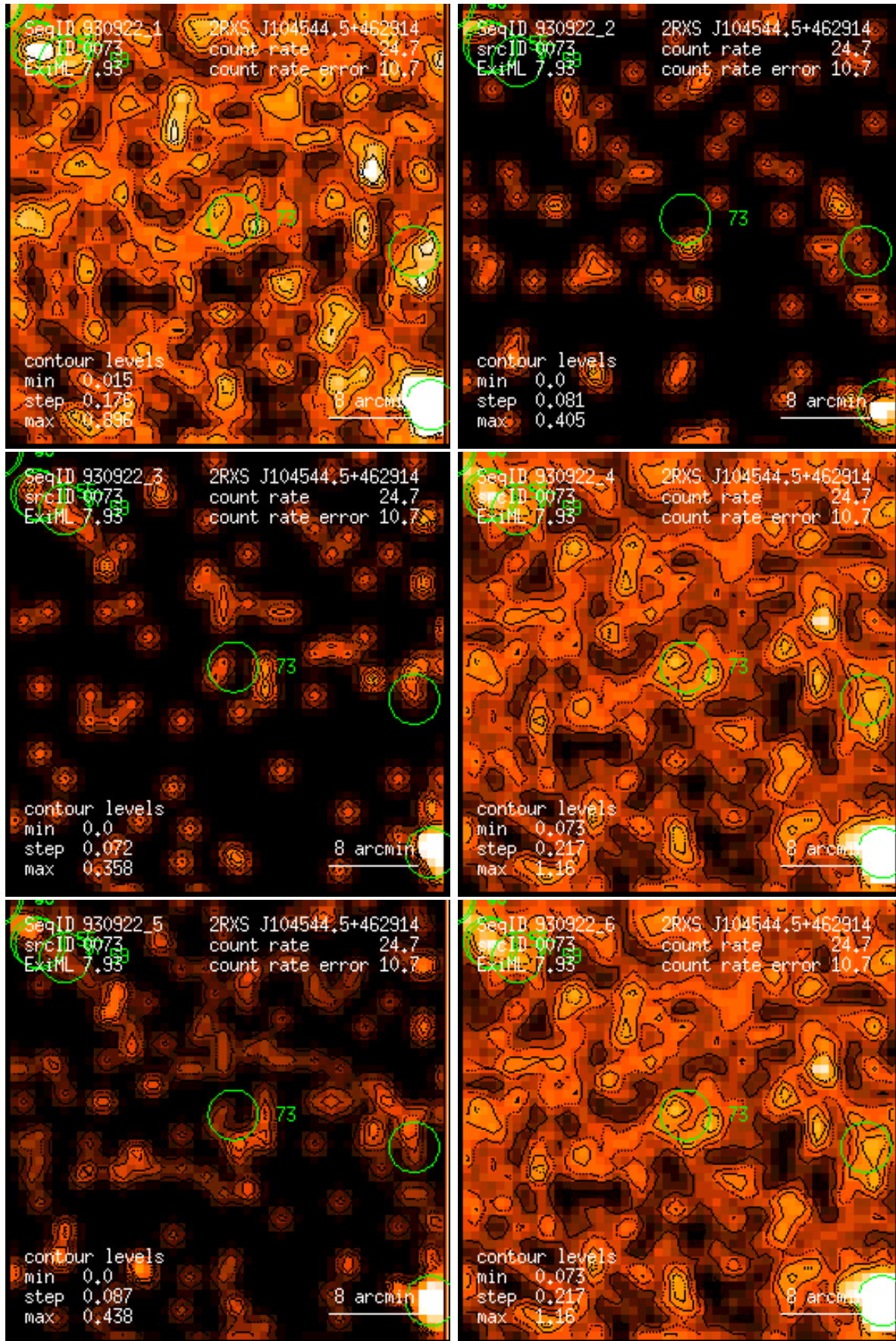
Figure 73: RASS 930922: detection 0073: band rate images, Gaussian filter: (1) PSPC channels 11 – 41, (2) 52 – 90, (3) 91 – 201, (4) 11 – 235, (5) 52 – 201, (6) 11 – 201. Broad band rates in counts/ks. Band rate contour levels in counts/ks/arcmin 2 .
