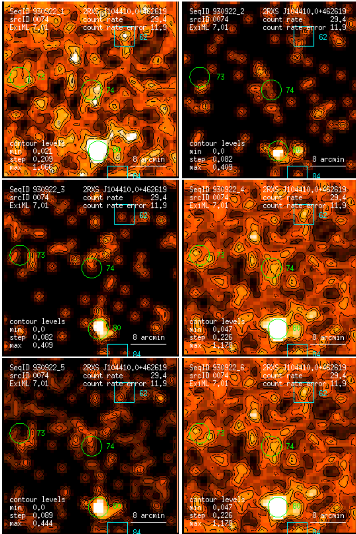
Figure 74: RASS 930922: detection 0074: band rate images, Gaussian filter: (1) PSPC channels 11 – 41, (2) 52 – 90, (3) 91 – 201, (4) 11 – 235, (5) 52 – 201, (6) 11 – 201. Broad band rates in counts/ks. Band rate contour levels in counts/ks/arcmin 2 .
