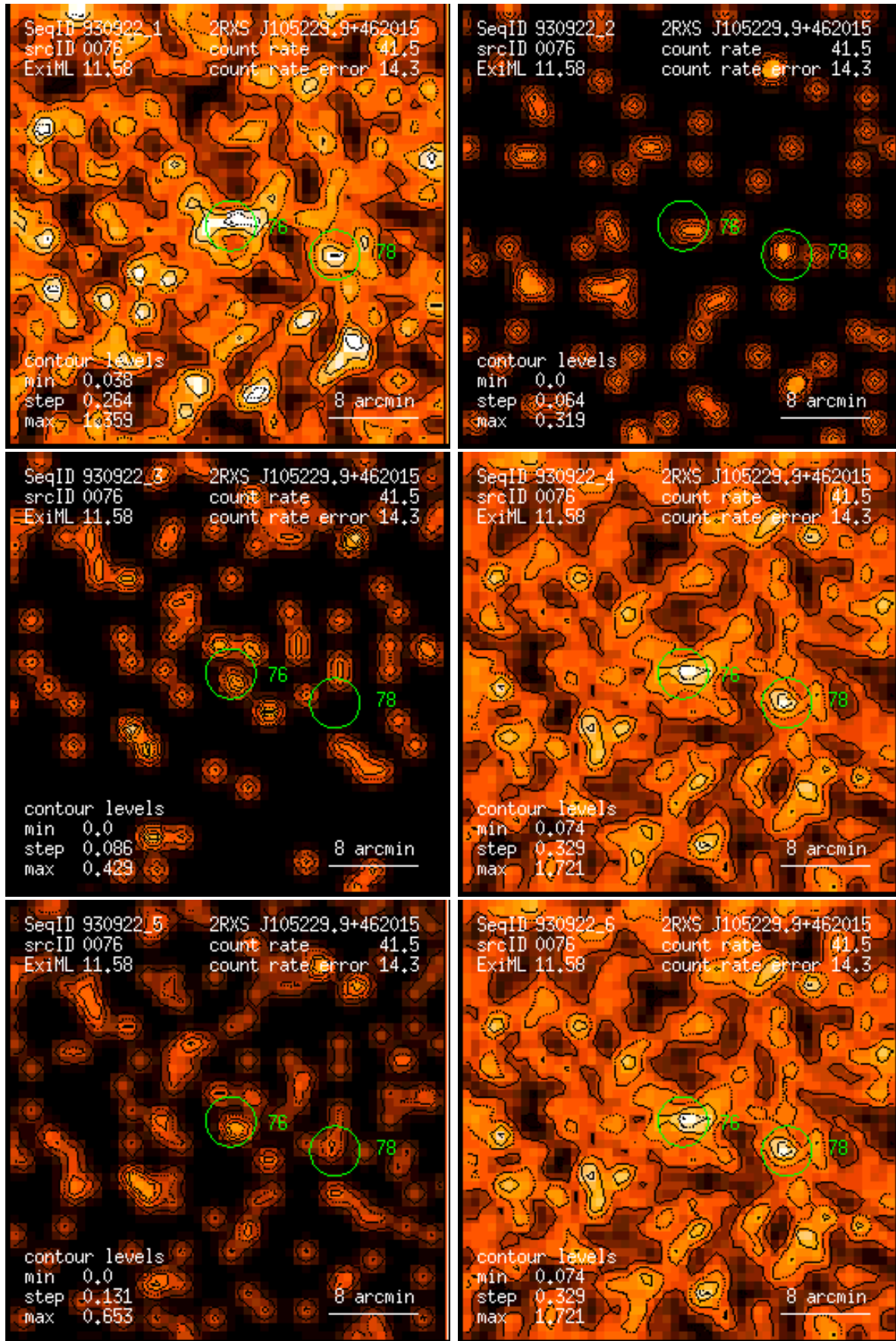
Figure 76: RASS 930922: detection 0076: band rate images, Gaussian filter: (1) PSPC channels 11 – 41, (2) 52 – 90, (3) 91 – 201, (4) 11 – 235, (5) 52 – 201, (6) 11 – 201. Broad band rates in counts/ks. Band rate contour levels in counts/ks/arcmin 2 .
