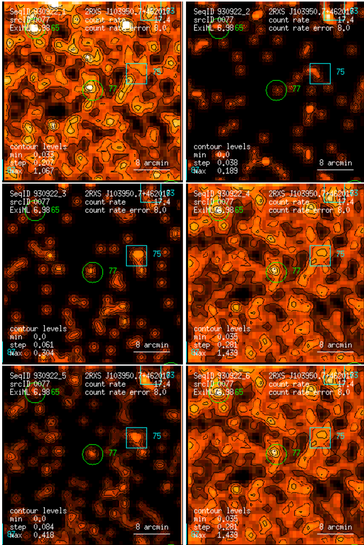
Figure 77: RASS 930922: detection 0077: band rate images, Gaussian filter: (1) PSPC channels 11 – 41, (2) 52 – 90, (3) 91 – 201, (4) 11 – 235, (5) 52 – 201, (6) 11 – 201. Broad band rates in counts/ks. Band rate contour levels in counts/ks/arcmin 2 .
