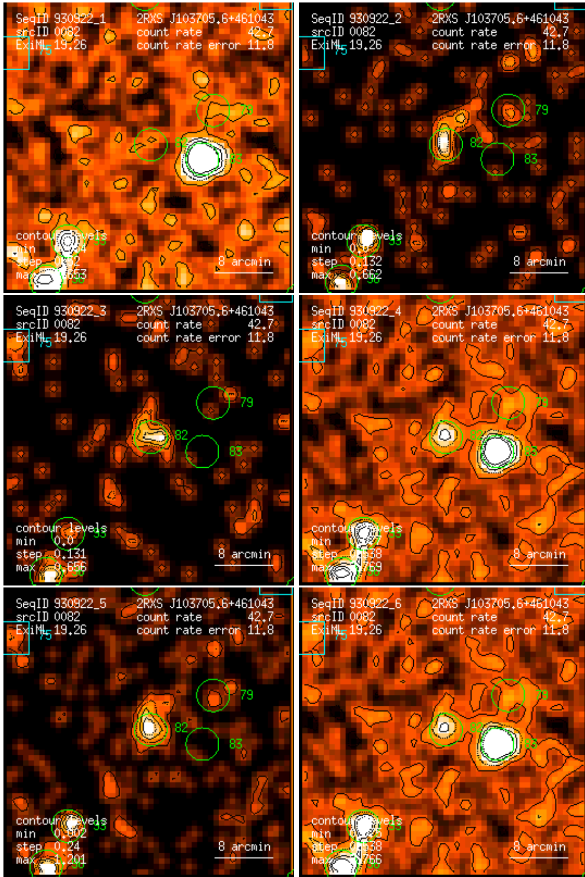
Figure 82: RASS 930922: detection 0082: band rate images, Gaussian filter: (1) PSPC channels 11 – 41, (2) 52 – 90, (3) 91 – 201, (4) 11 – 235, (5) 52 – 201, (6) 11 – 201. Broad band rates in counts/ks. Band rate contour levels in counts/ks/arcmin 2 .
