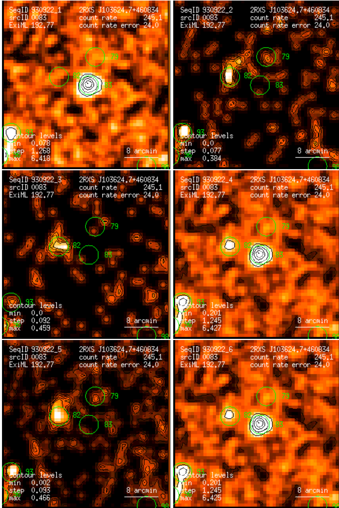
Figure 83: RASS 930922: detection 0083: band rate images, Gaussian filter: (1) PSPC channels 11 – 41, (2) 52 – 90, (3) 91 – 201, (4) 11 – 235, (5) 52 – 201, (6) 11 – 201. Broad band rates in counts/ks. Band rate contour levels in counts/ks/arcmin 2 .
