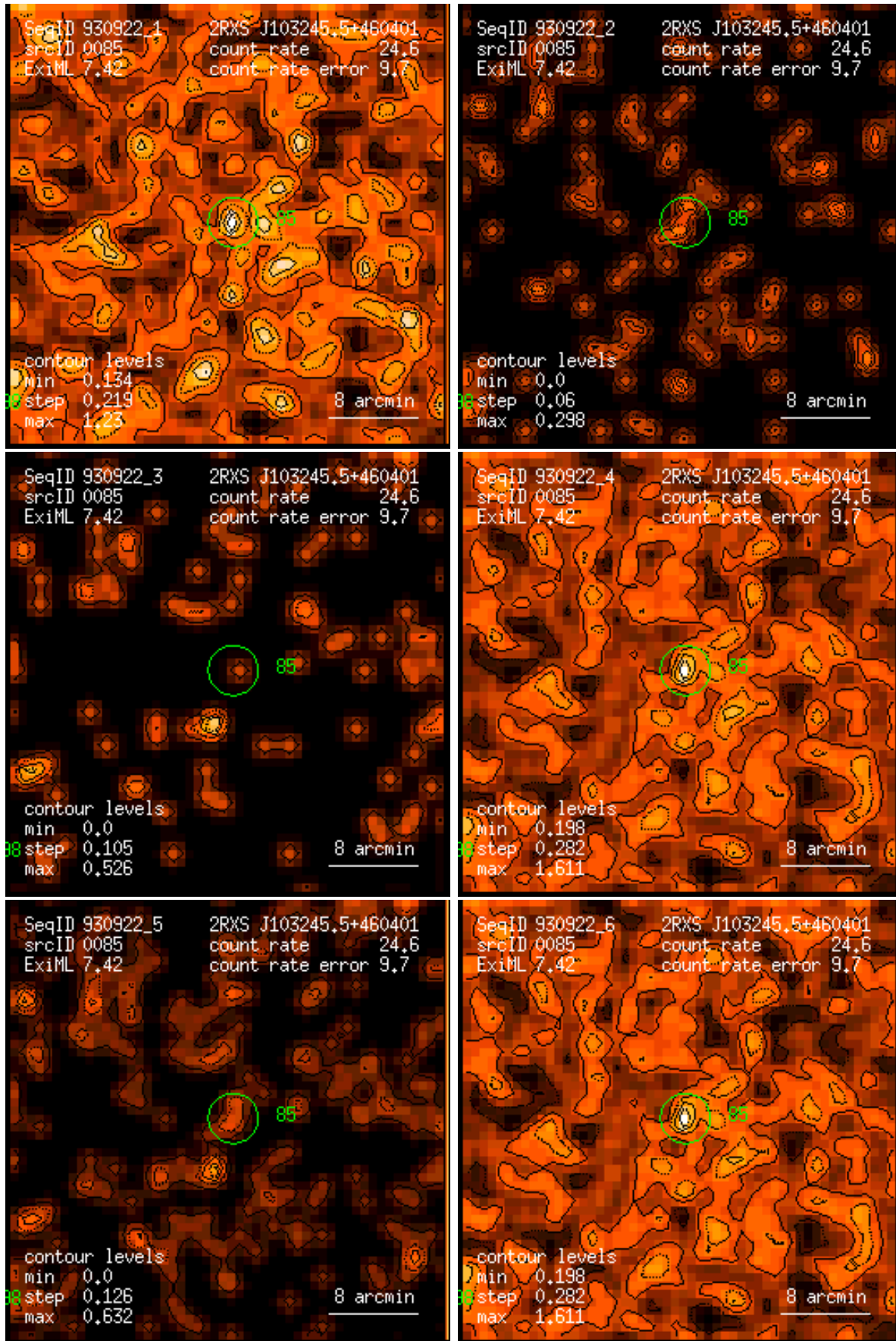
Figure 85: RASS 930922: detection 0085: band rate images, Gaussian filter: (1) PSPC channels 11 – 41, (2) 52 – 90, (3) 91 – 201, (4) 11 – 235, (5) 52 – 201, (6) 11 – 201. Broad band rates in counts/ks. Band rate contour levels in counts/ks/arcmin 2 .
