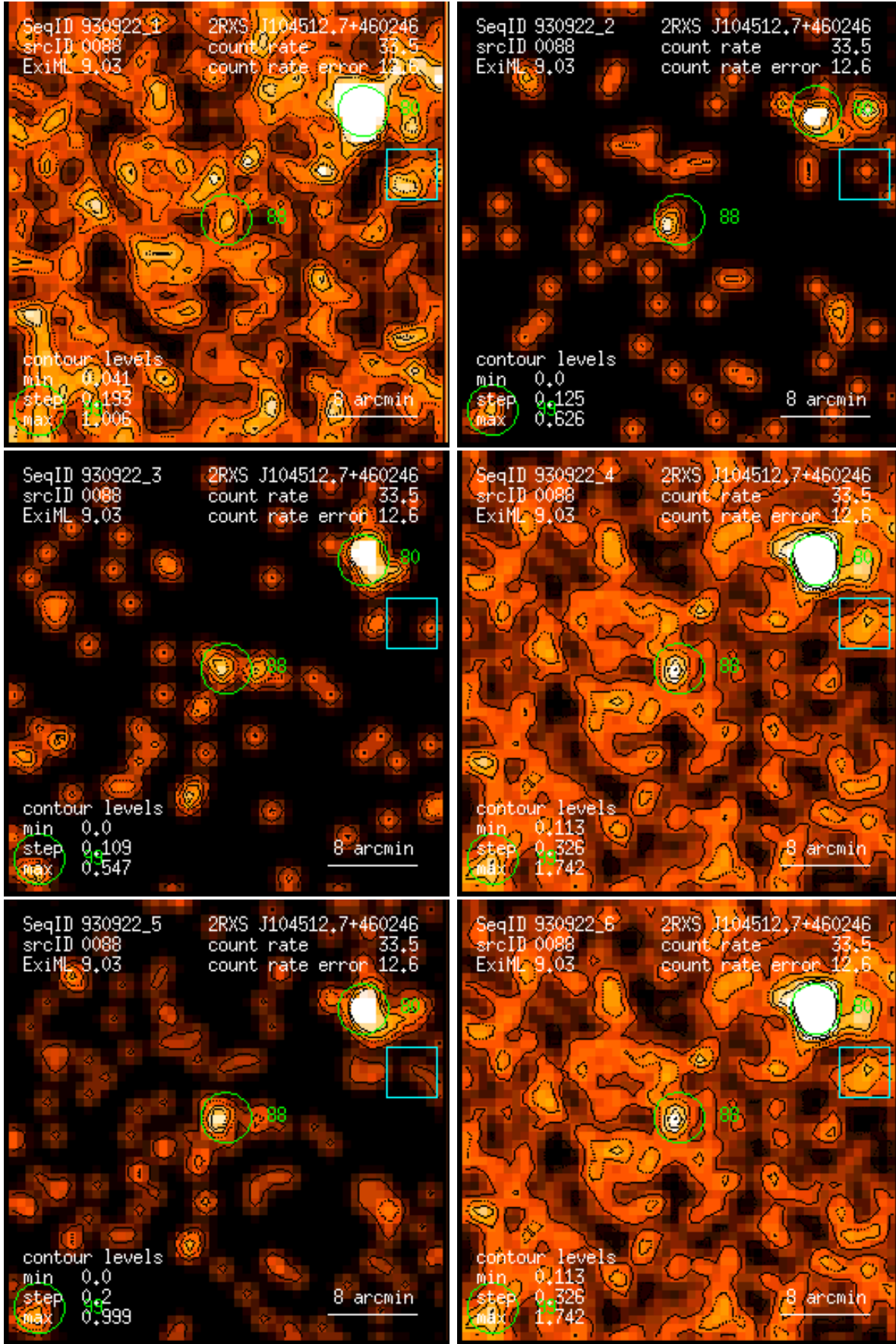
Figure 88: RASS 930922: detection 0088: band rate images, Gaussian filter: (1) PSPC channels 11 – 41, (2) 52 – 90, (3) 91 – 201, (4) 11 – 235, (5) 52 – 201, (6) 11 – 201. Broad band rates in counts/ks. Band rate contour levels in counts/ks/arcmin 2 .
